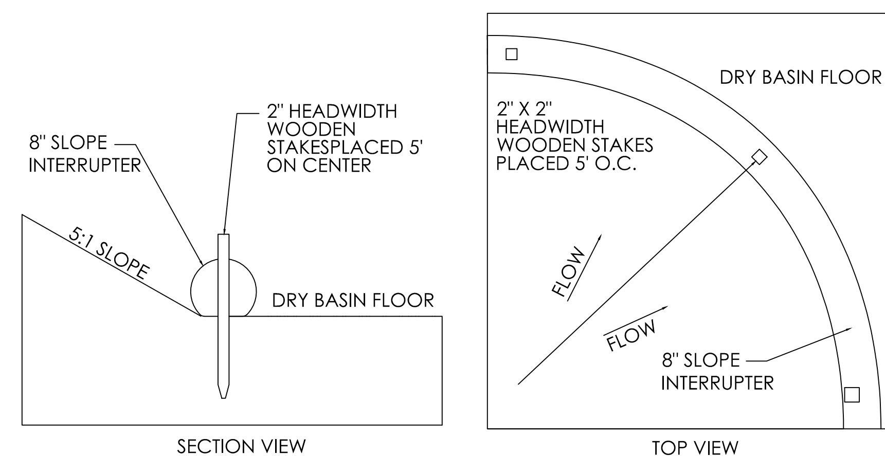
SEDIMENT LOGS (WATTLES)
