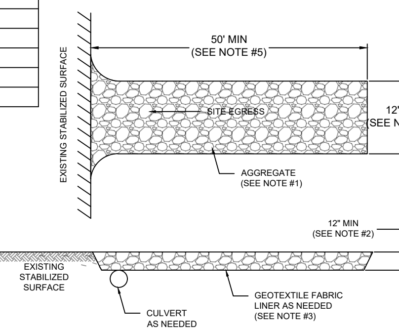
STONE TRACKING PAD DETAIL
