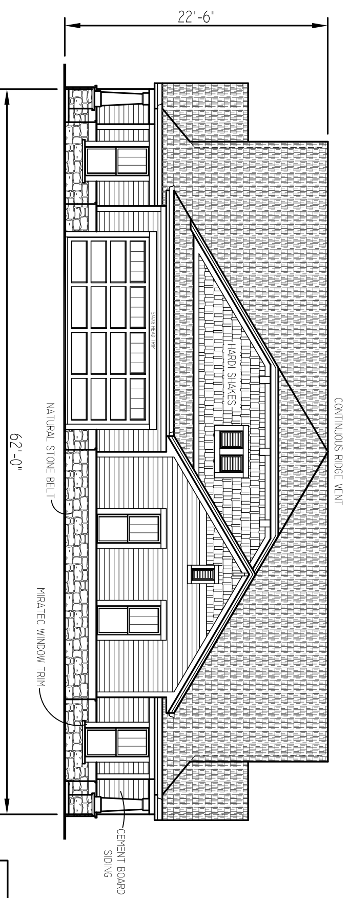
FRONT ELEVATION
