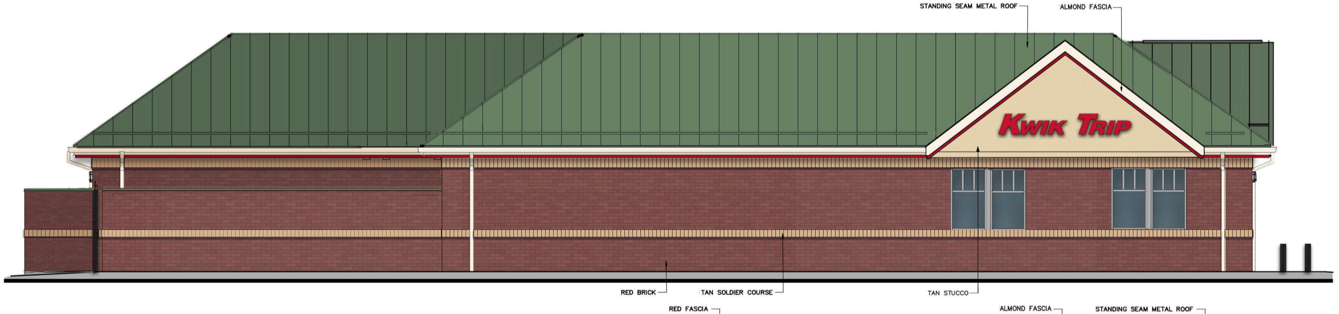
3 REAR ELEVATION 3/16" = 1'-0"
