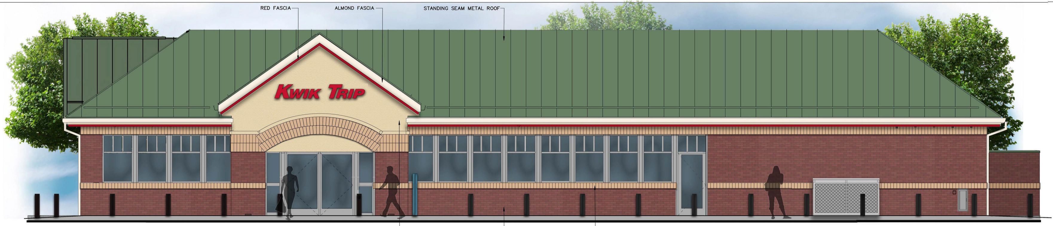
1 FRONT ELEVATION 1/4" = 1'-0"
