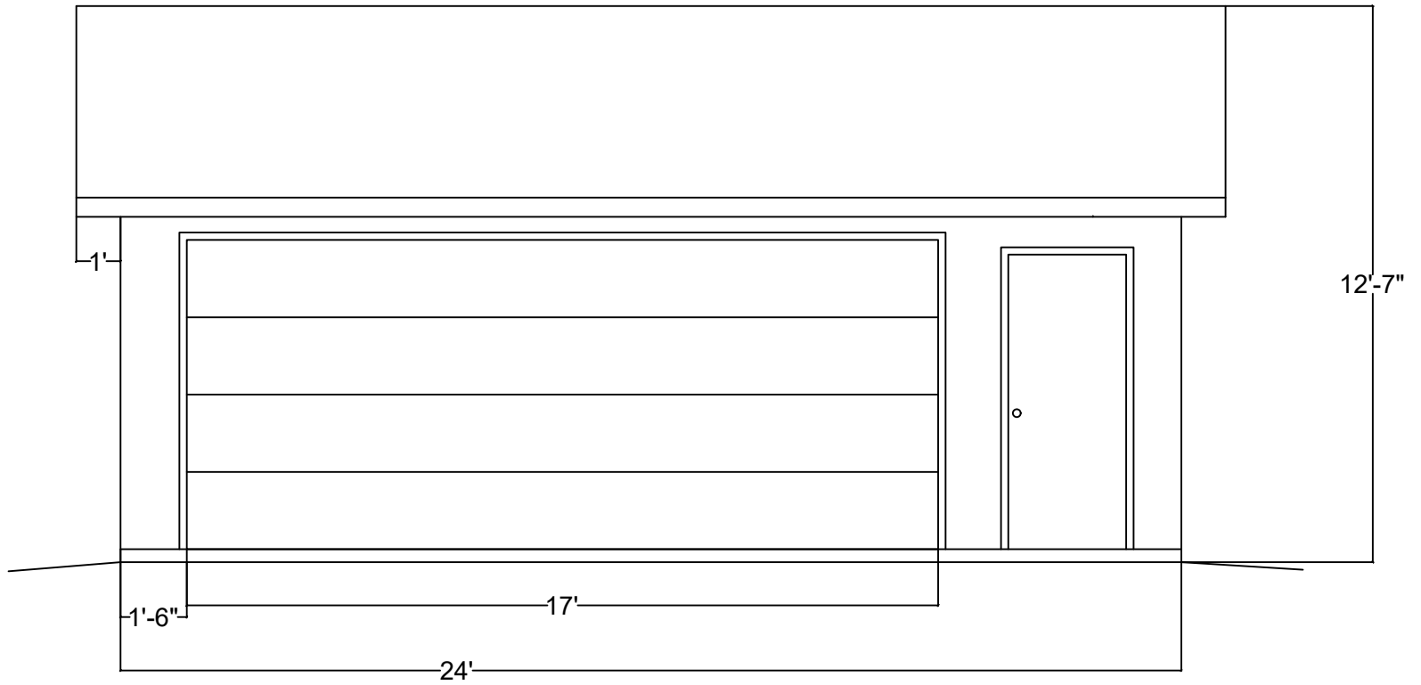
East Elevation
