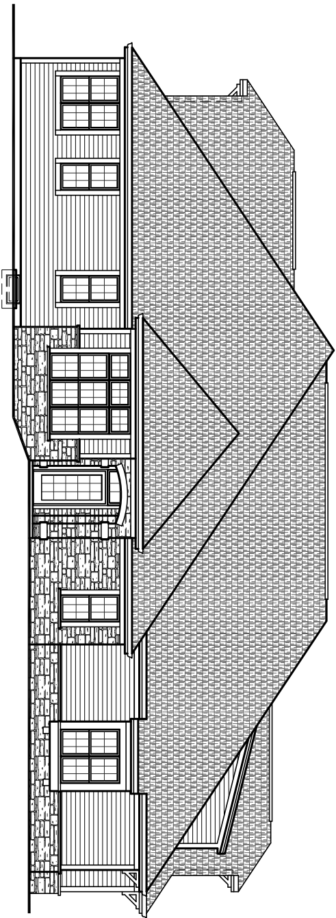
LEFT ELEVATION
