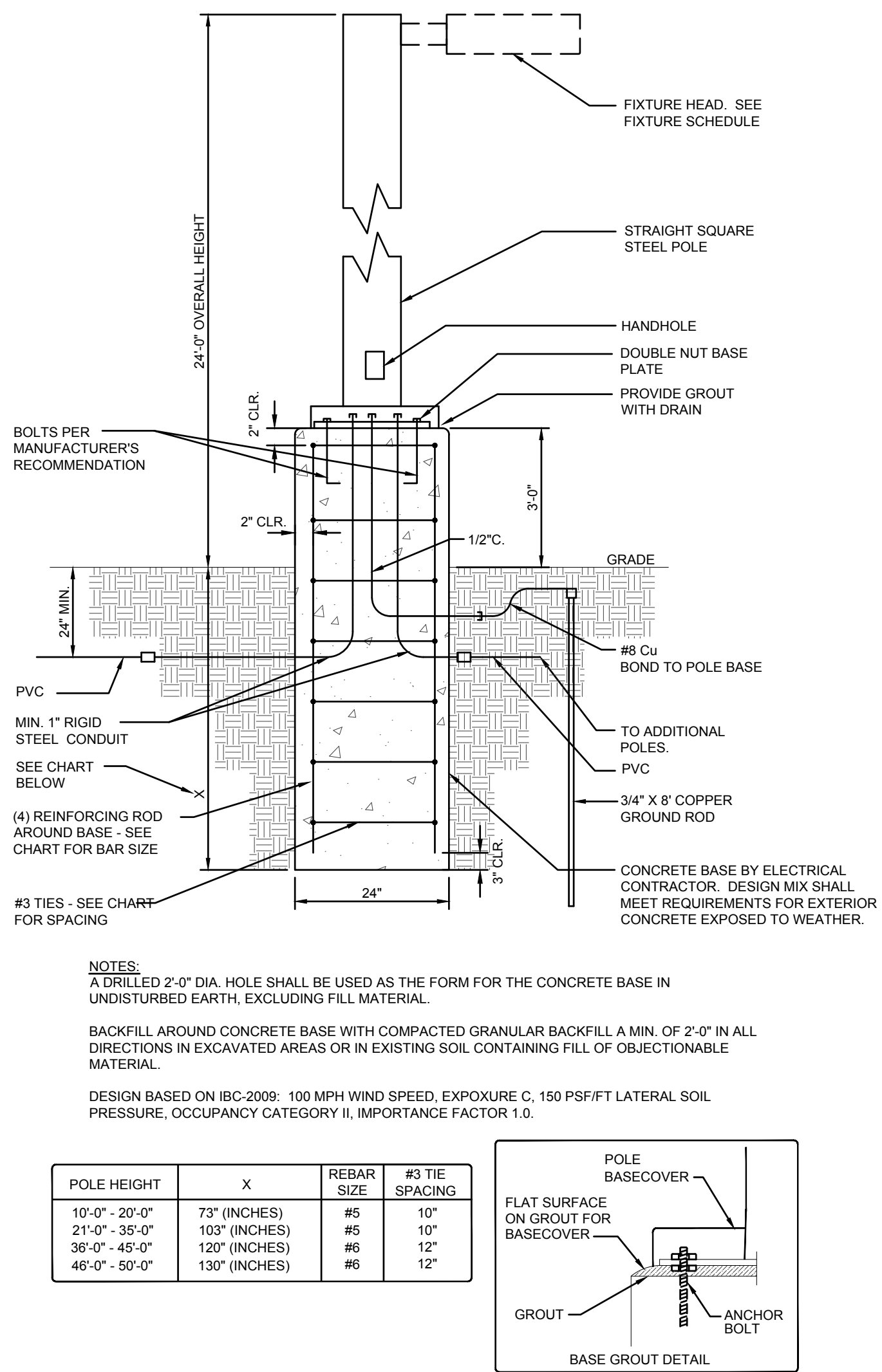
LIGHT POLE DETAIL NO SCALE
