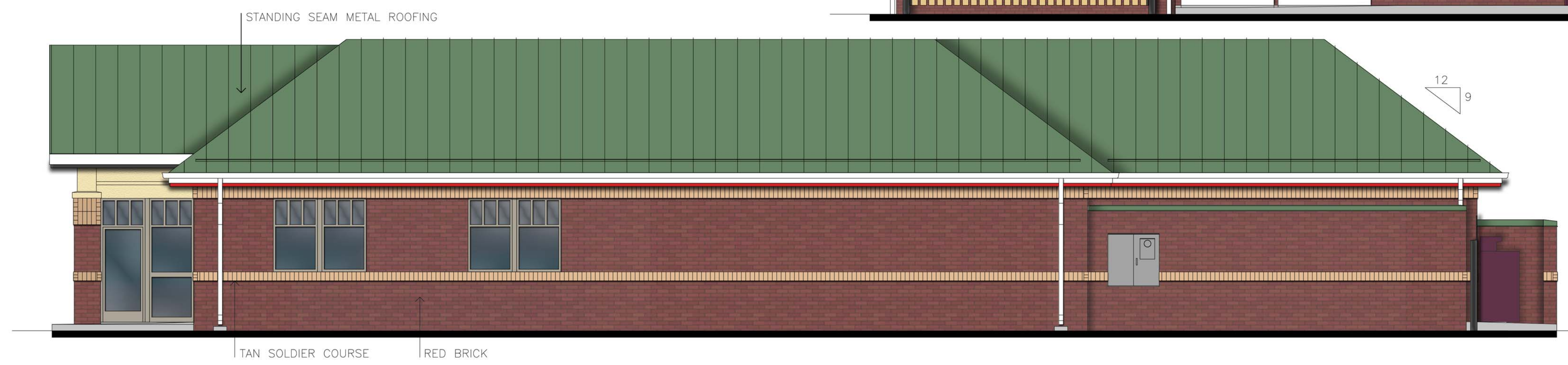
RIGHT ELEVATION 3/16" = 1'-0"
