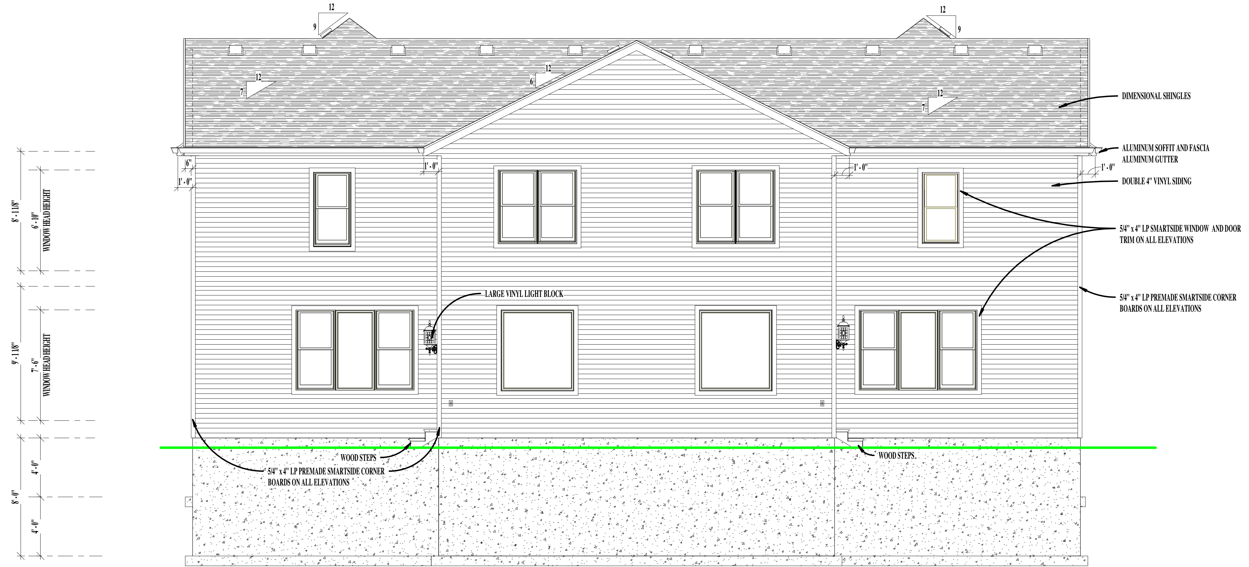
REAR ELEVATION
