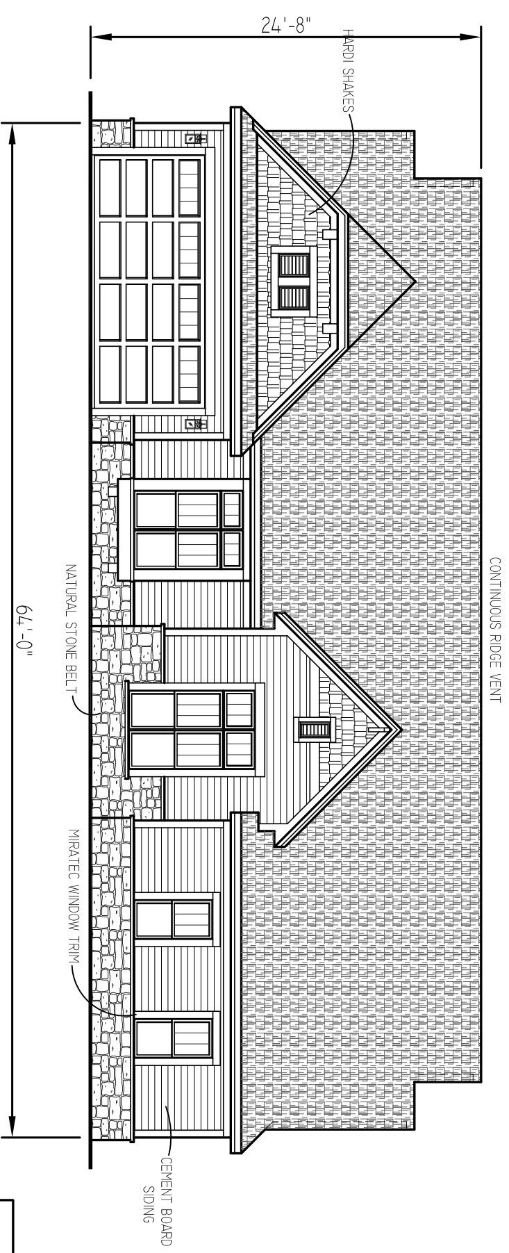
FRONT ELEVATION
