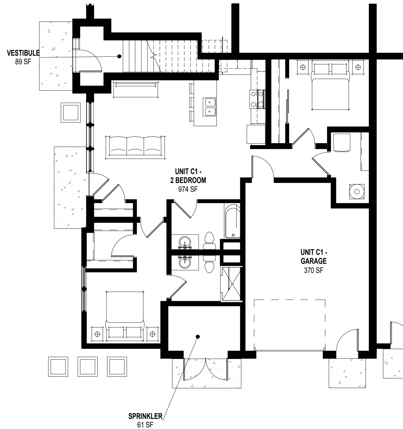
2 FIRST FLOOR - 2 BEDROOM - CORNER 1/8" = 1'-0"
