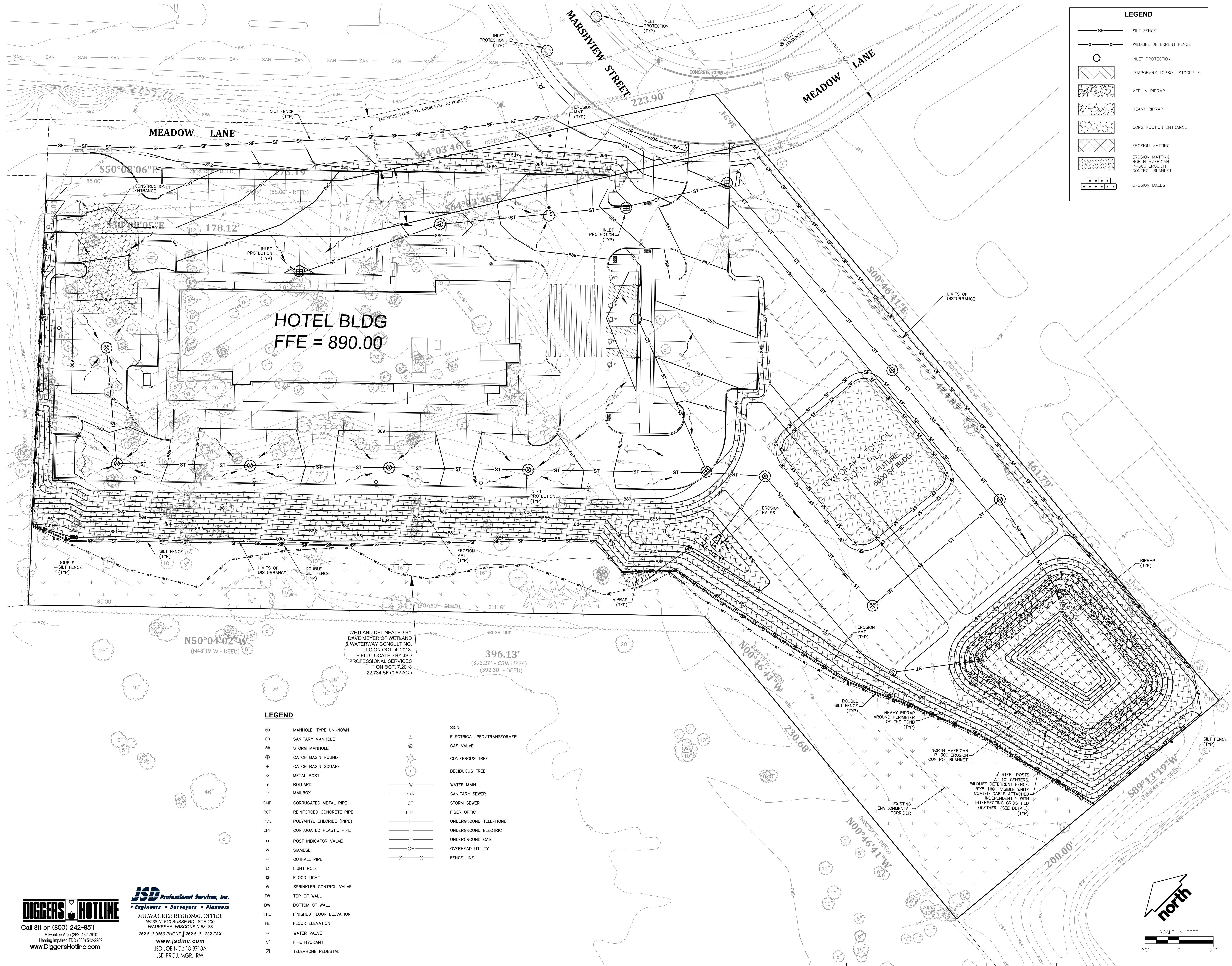
EROSION CONTROL PLAN 1" = 20'-0"
