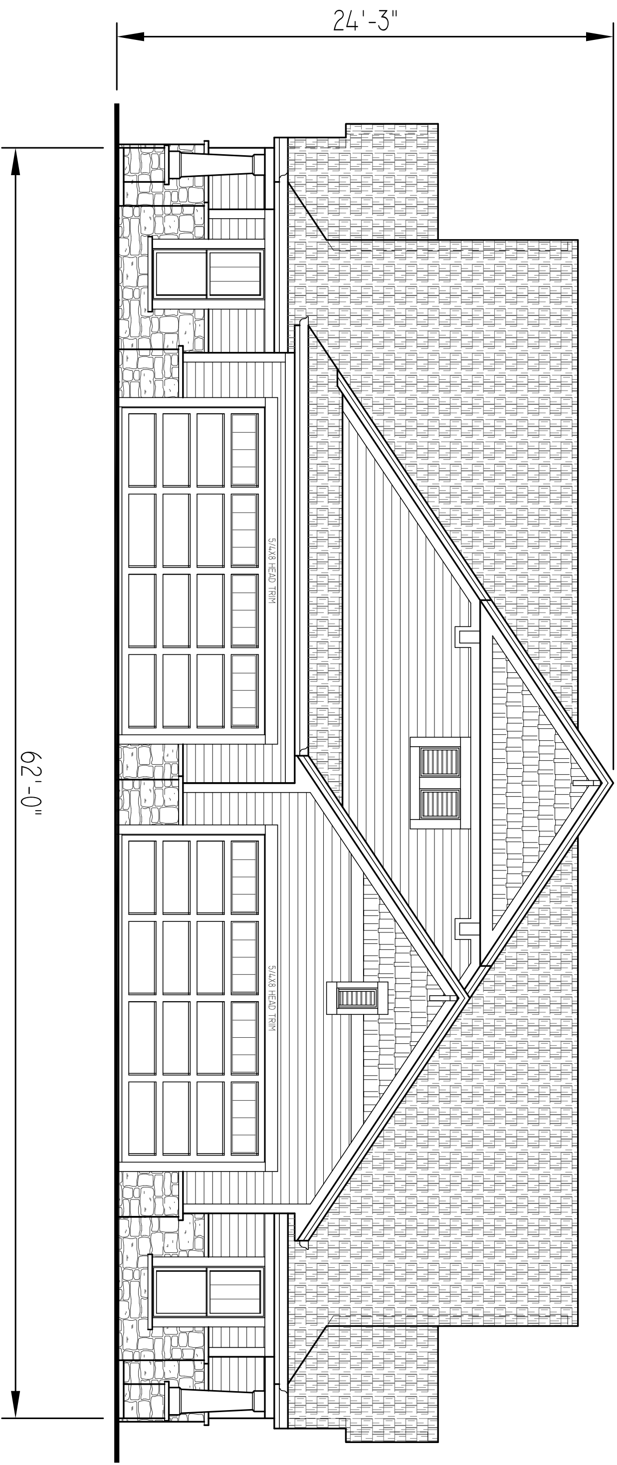
FRONT ELEVATION
