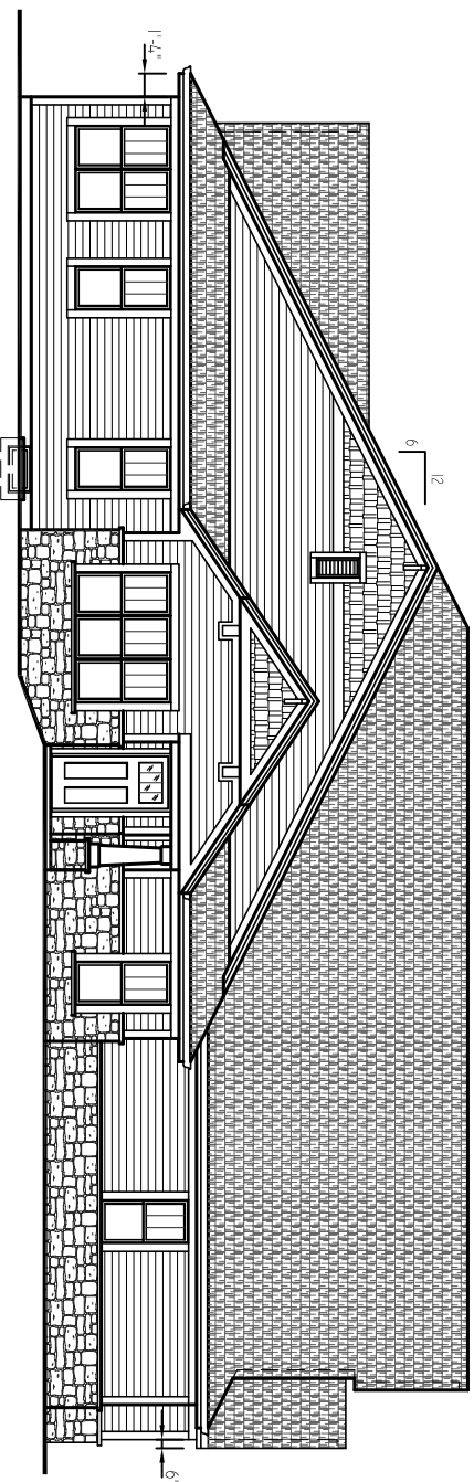
LEFT ELEVATION
