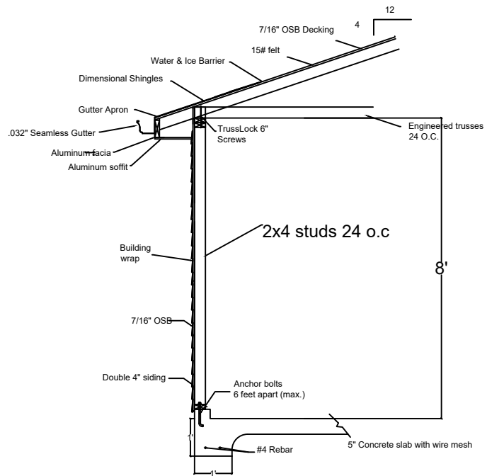
Cross Section (Typical)
