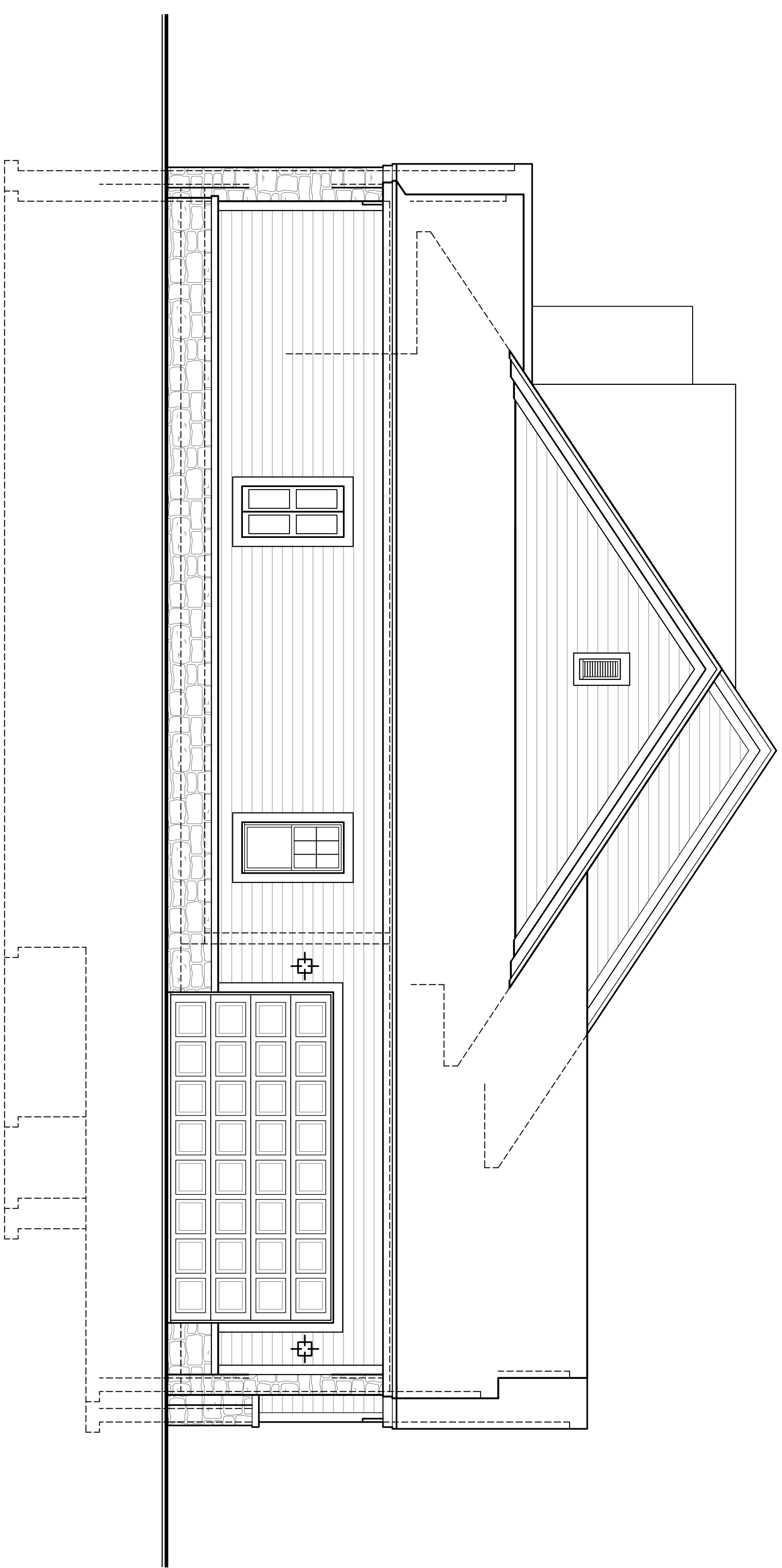
LEFT SIDE ELEVATION
