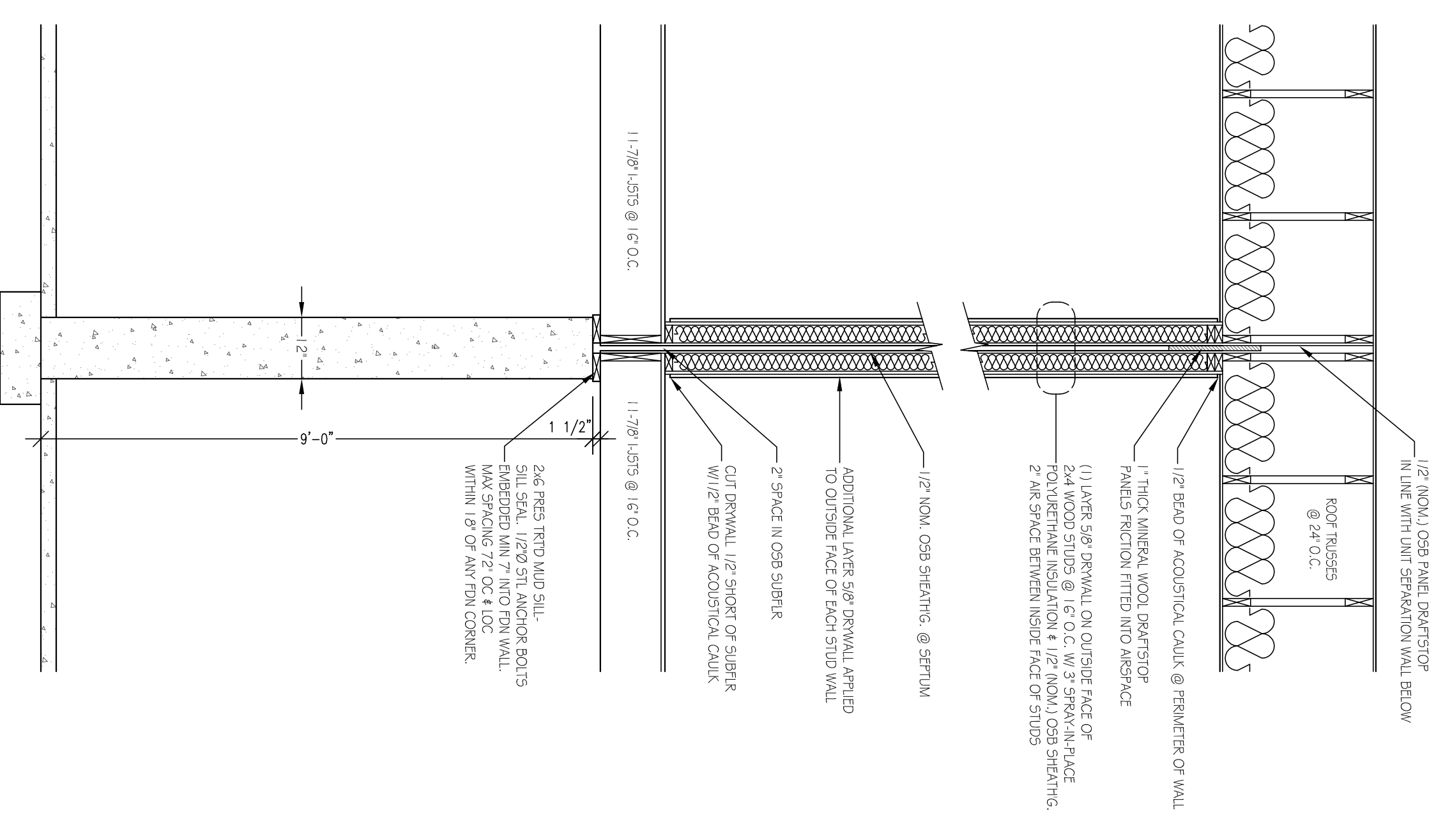
UNIT SEPARATION ASSEMBLY SCALE: 1/2" = 1'-0"
