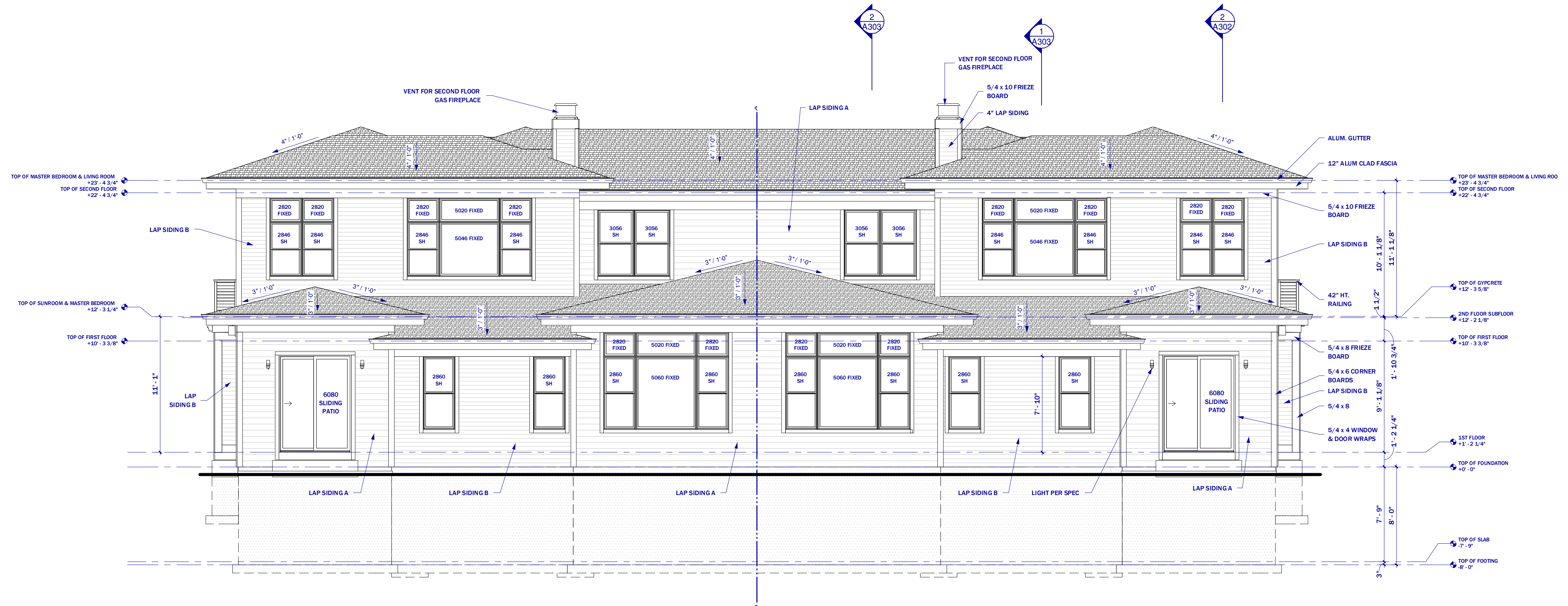
2 REAR ELEVATION SCALE: 1/4" = 1'-0"
