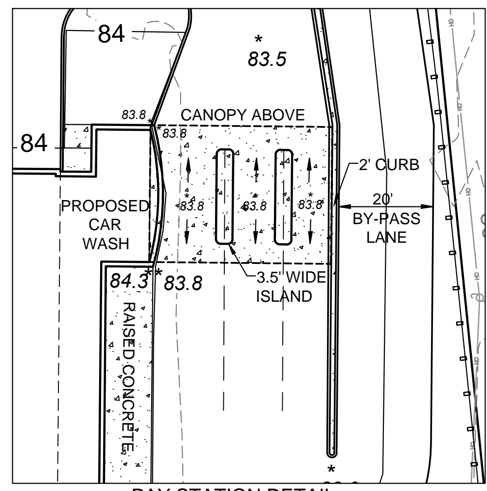
PAY STATION DETAIL SCALE = 1" - 20'
