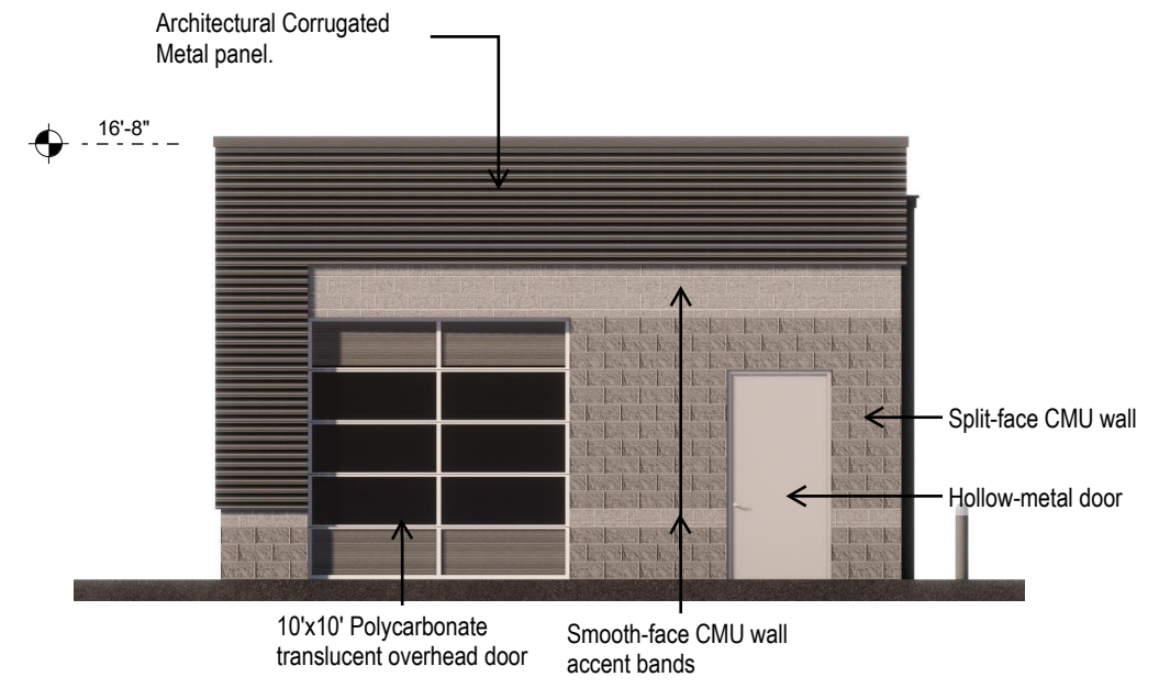
East Elevation
