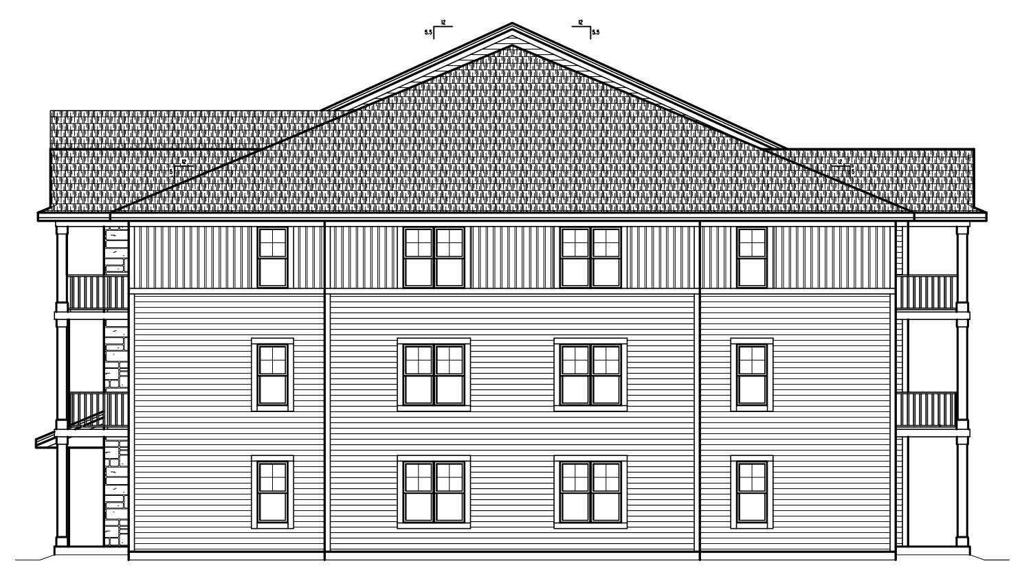
WEST ELEVATION
