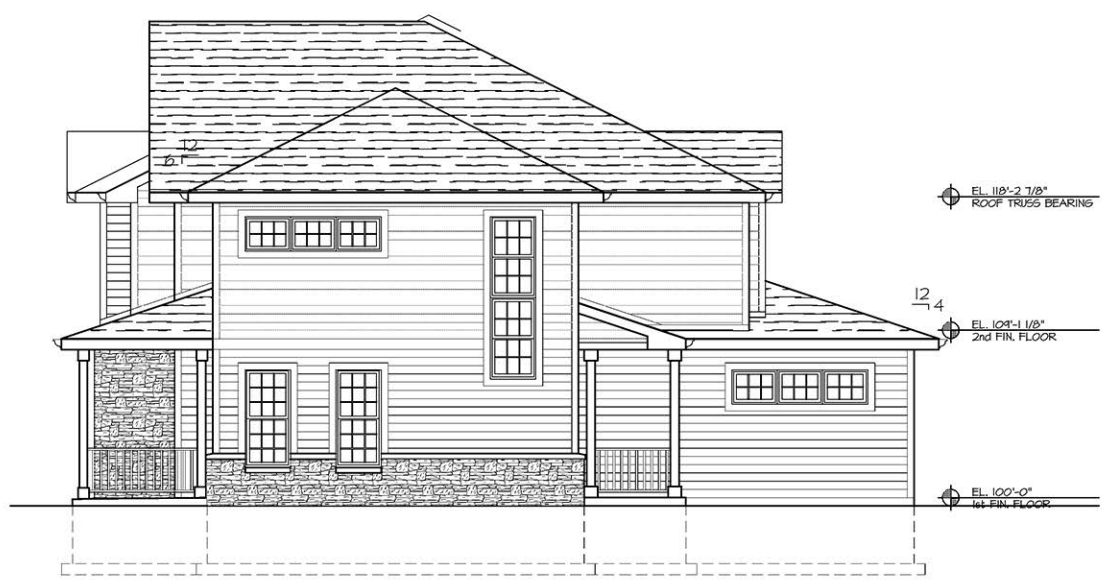
NORTHEAST ELEVATION 3/16" = 1'-0"
