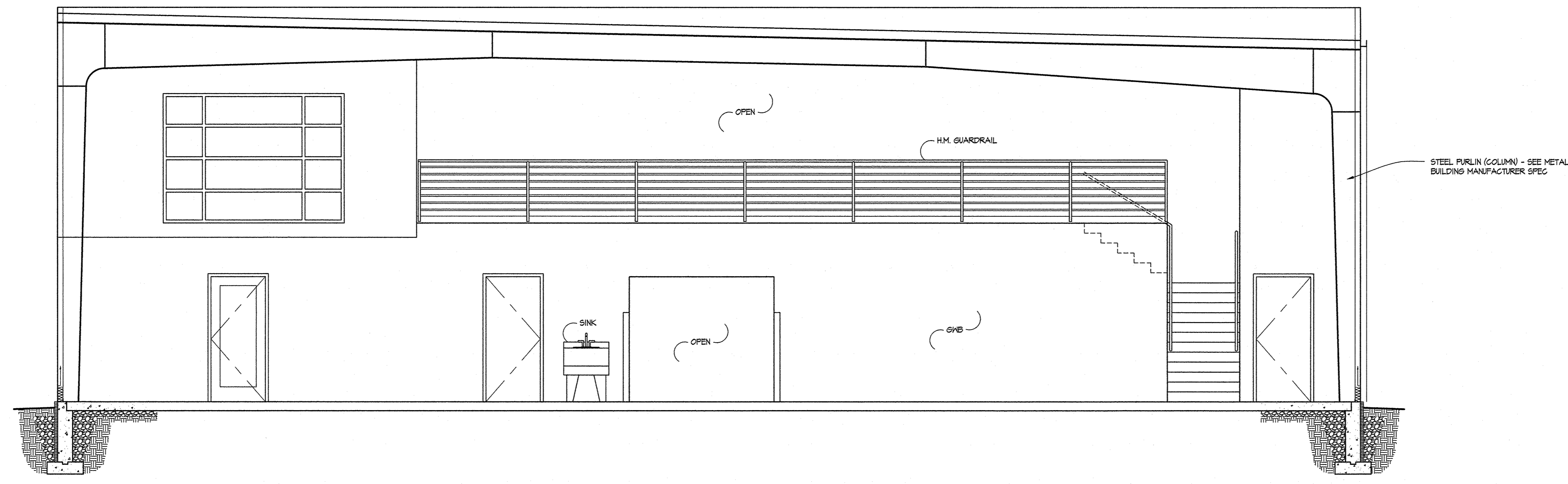
1 BUILDING SECTION @ SHOP
