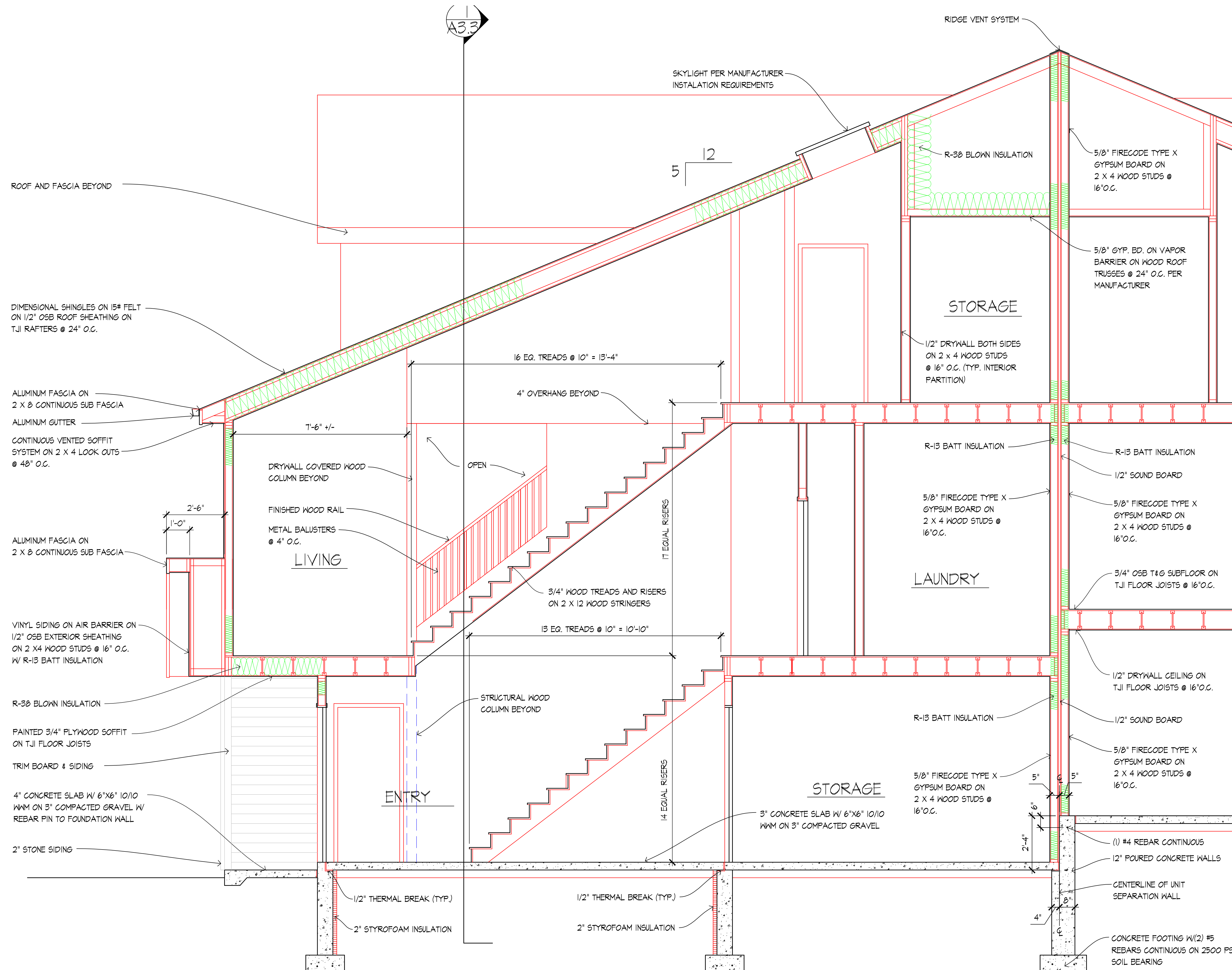
BUILDING SECTION SCALE: 1/2" = 1'-0"
