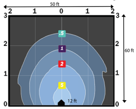
WS 38 (12 Feet Mounting)
