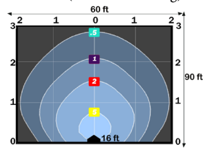
WM 81 (16 Feet Mounting)
