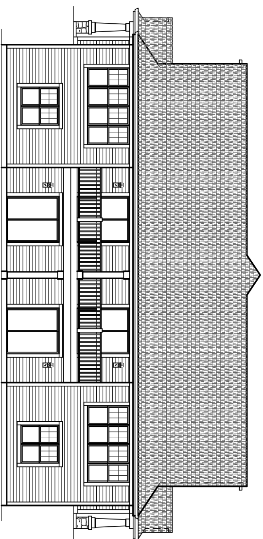
REAR ELEVATION
