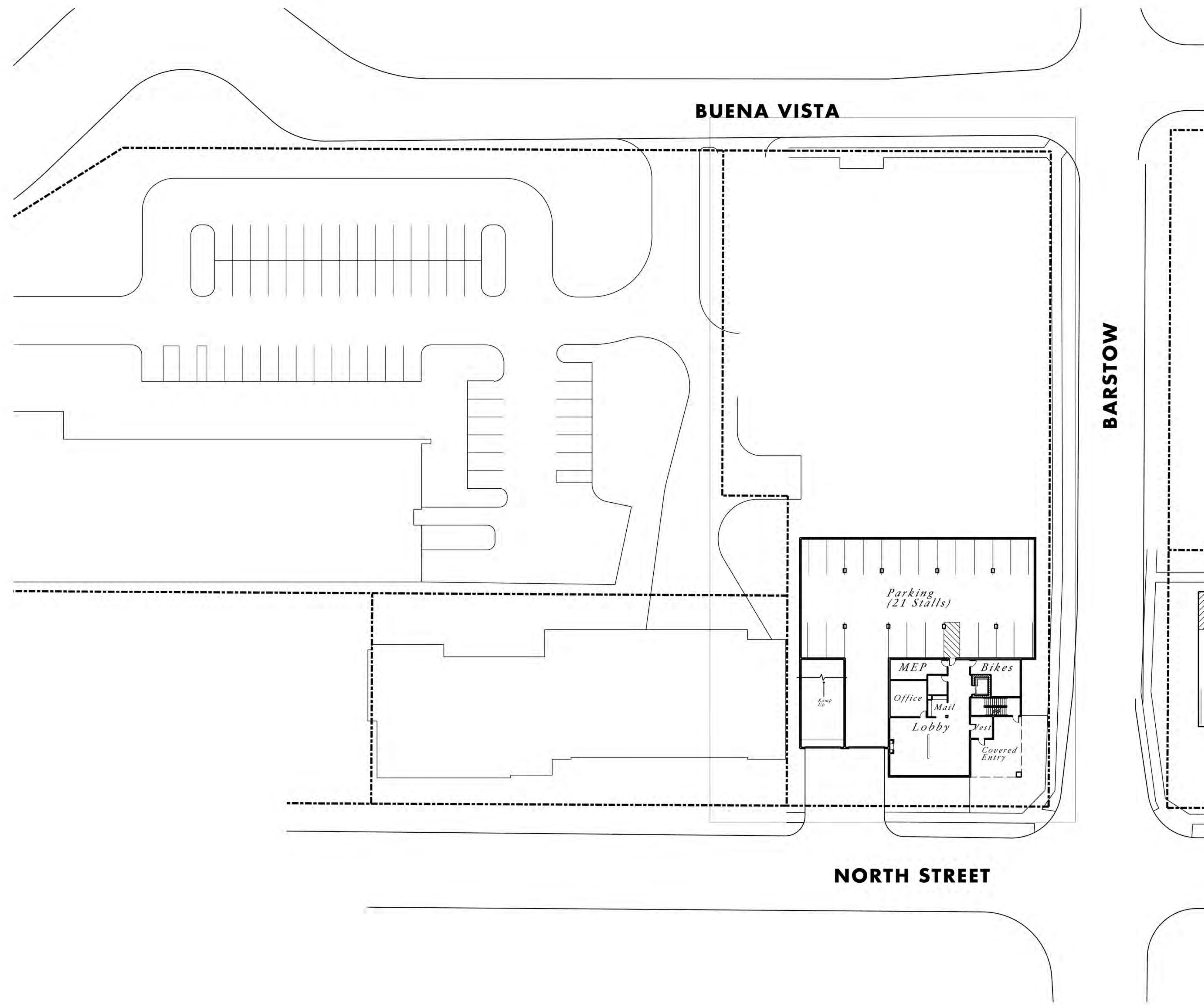
LOWER LEVEL PARKING/FIRST FLOOR PLAN 12,391 SF | 21 Cars
