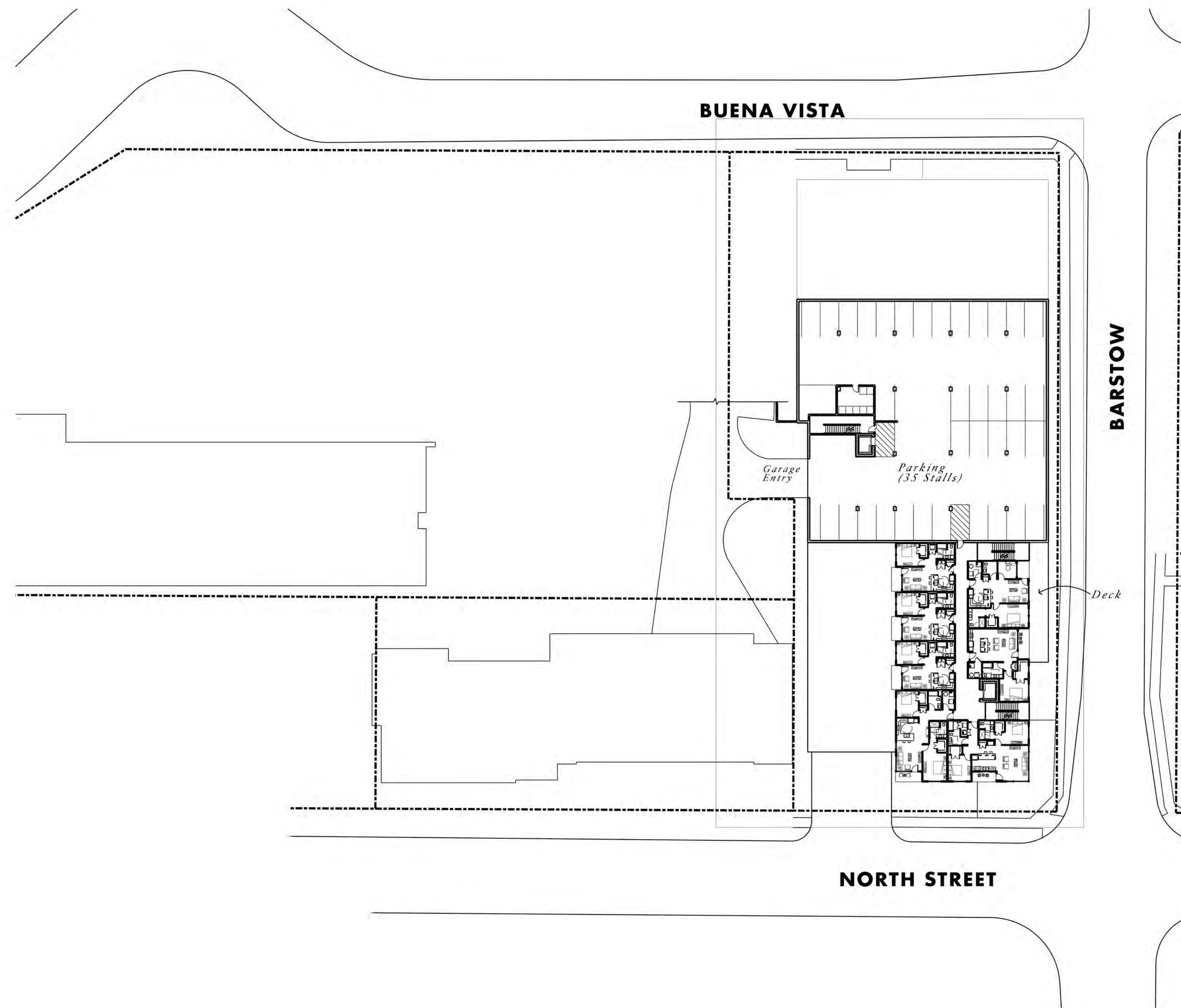
THIRD FLOOR PLAN 20,086 SF | 35 Cars | 7 Apartments
