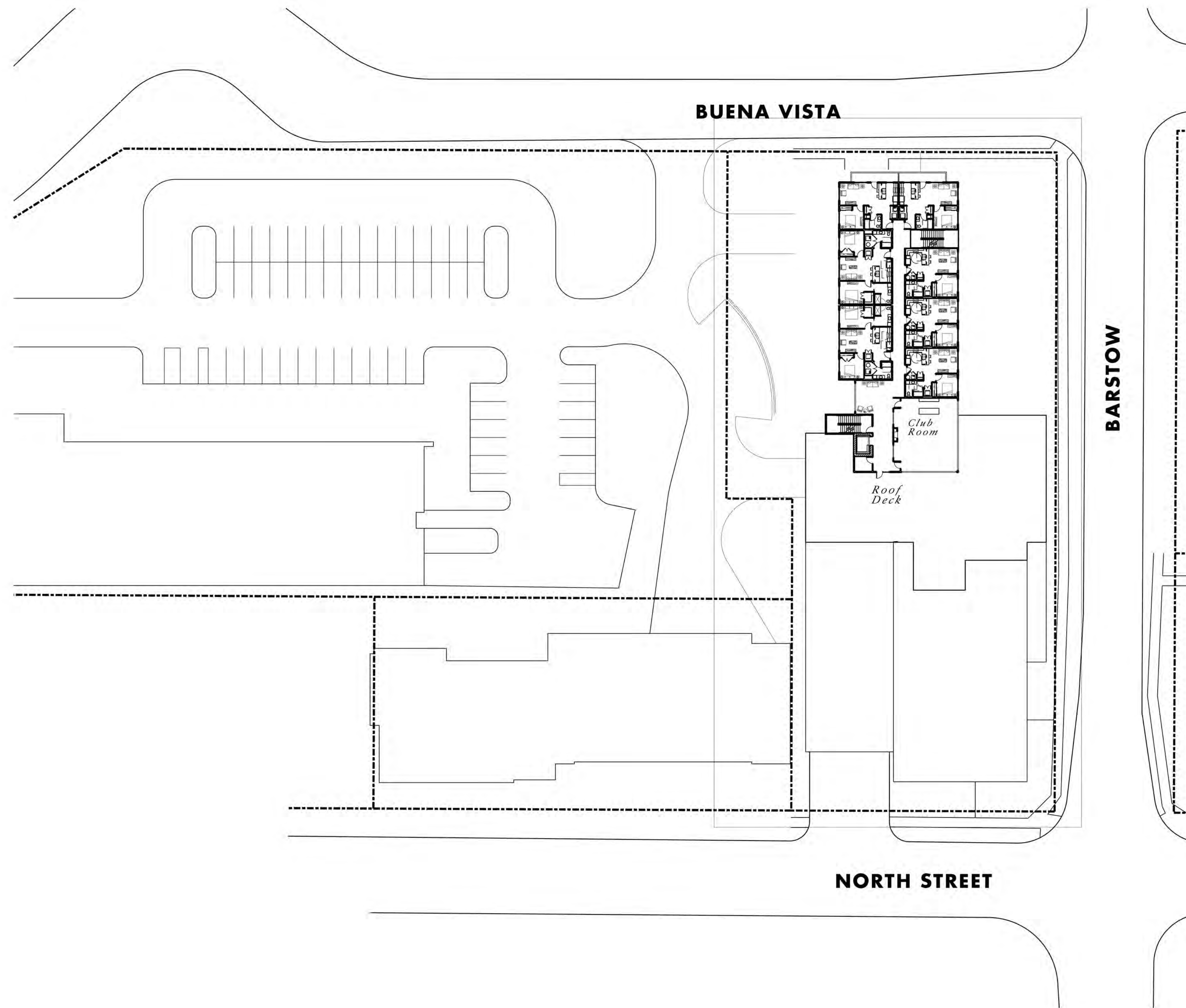
EIGHTH FLOOR PLAN 8,101 SF | 7 Apartments
