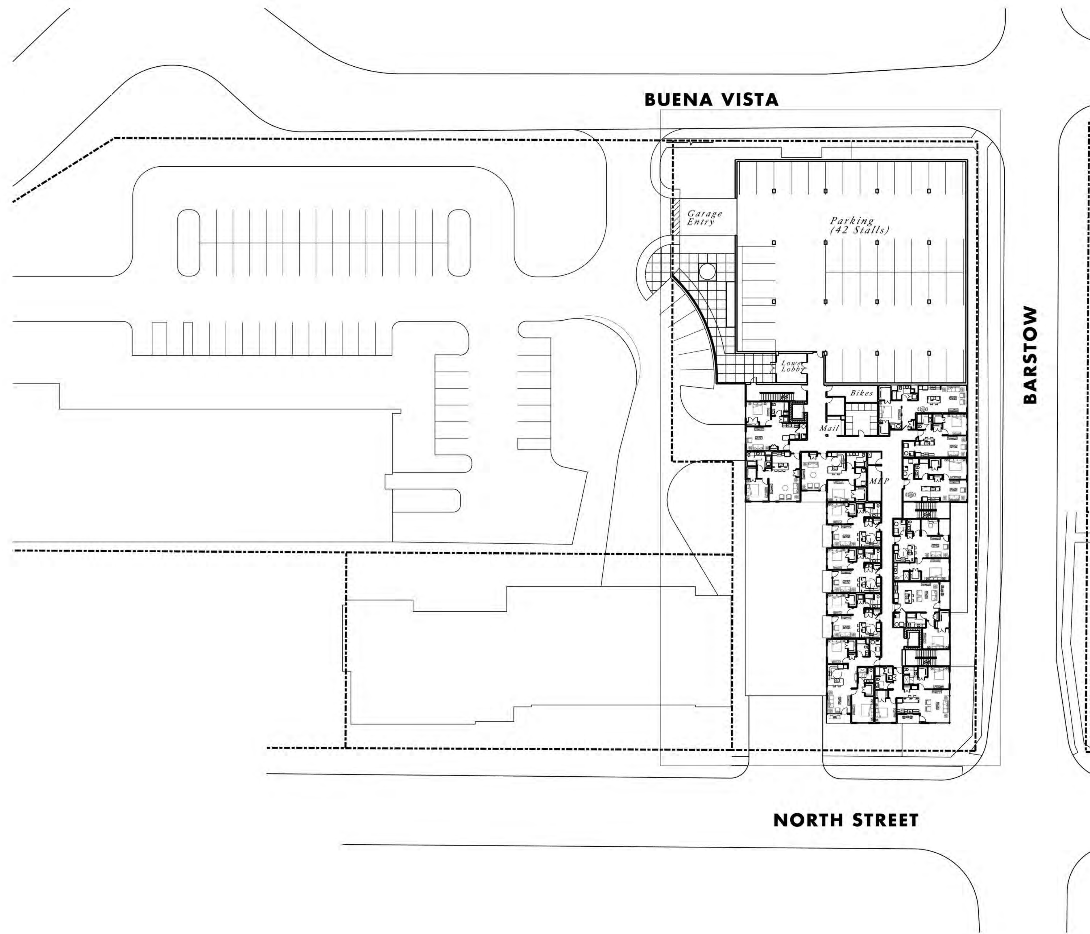
FOURTH FLOOR PLAN 30,605 SF | 42 Cars | 13 Apartments
