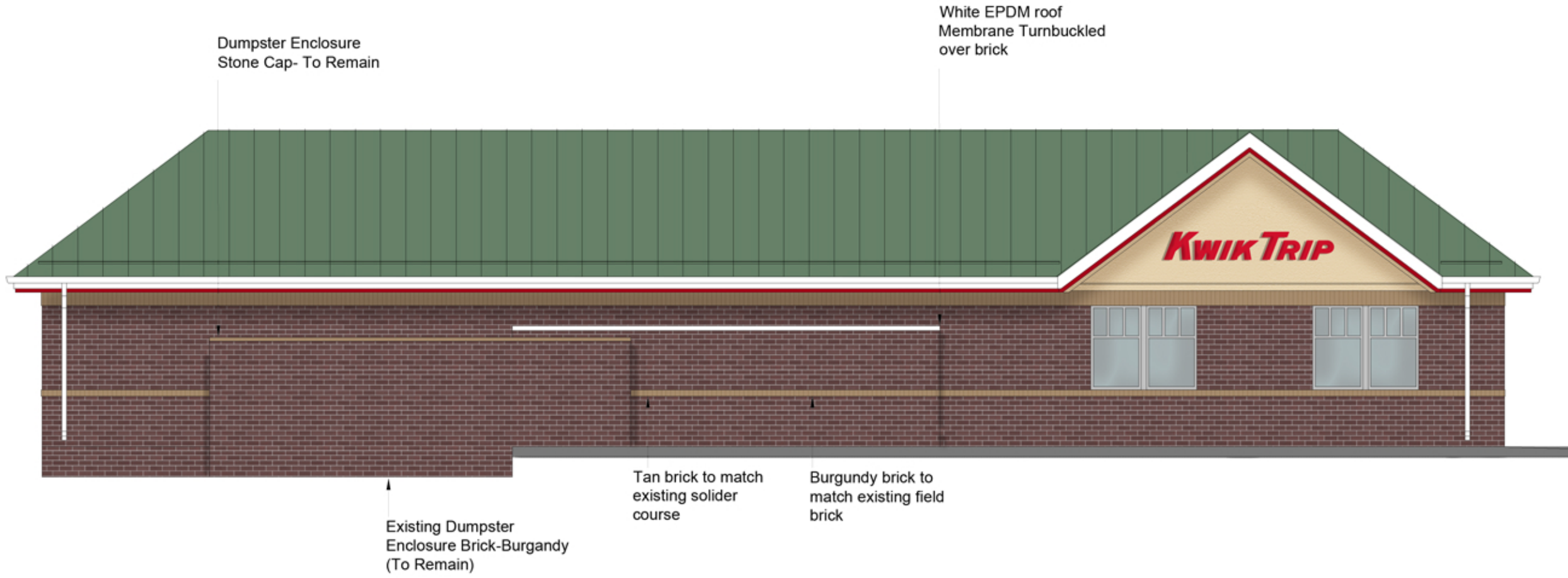
SOUTH ELEVATION
