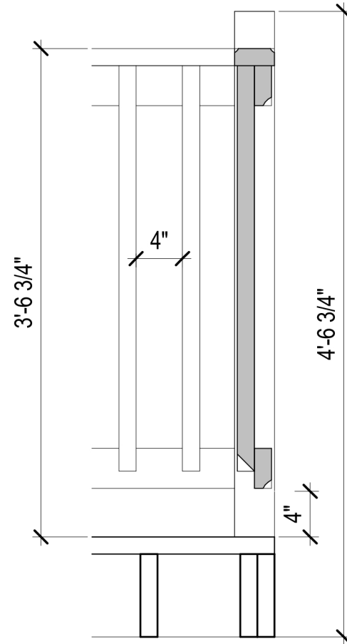
2 HANDRAIL SECTION 1" = 1'-0"
