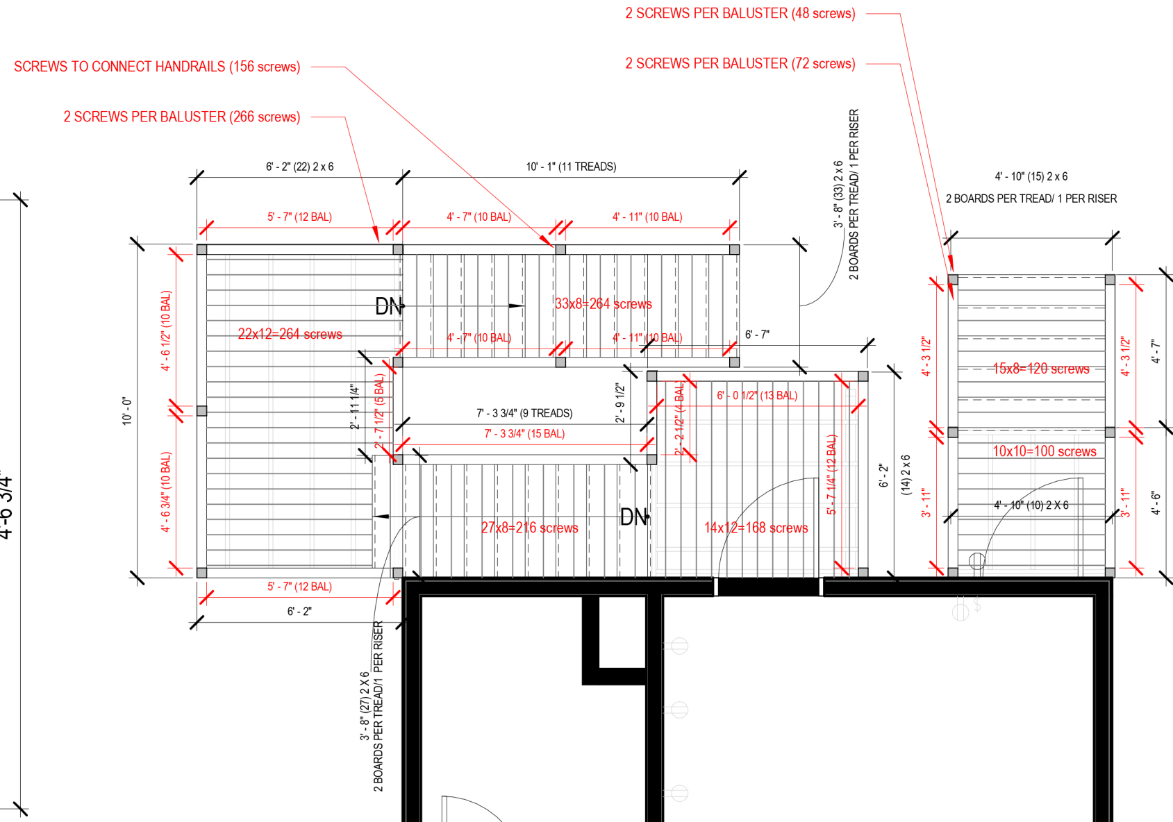
1 FLOOR PLAN - LEVEL 02 - STAIR 1/4" = 1'-0"
