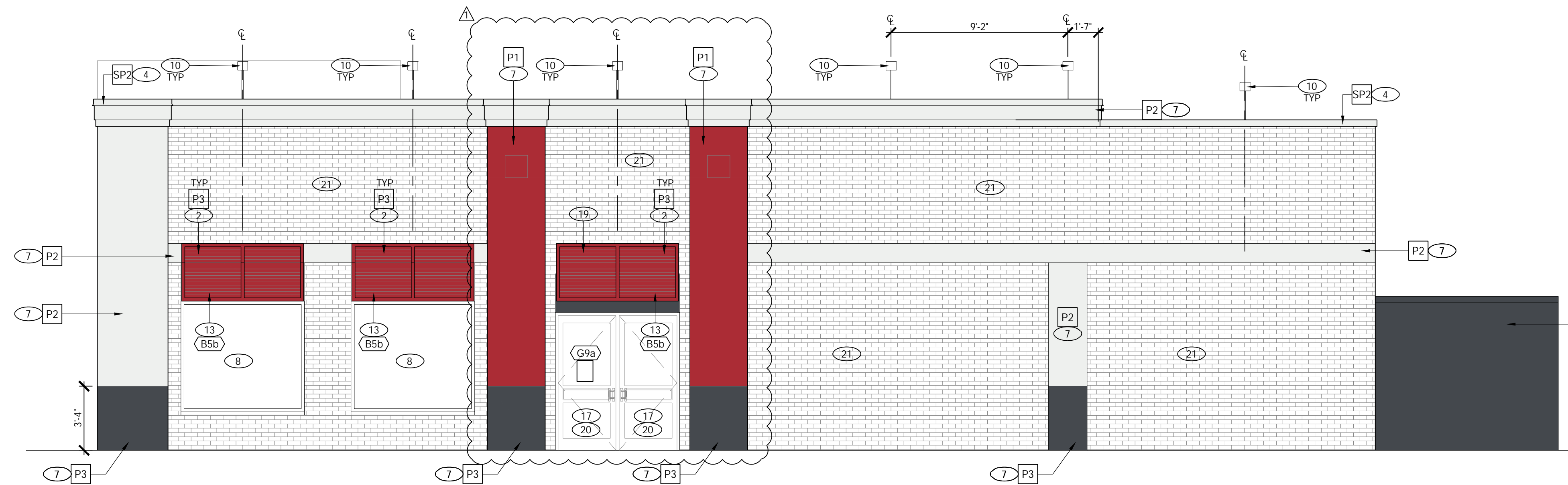
3 - ENTRY ELEVATION Scale: 1/4" = 1'-0"
