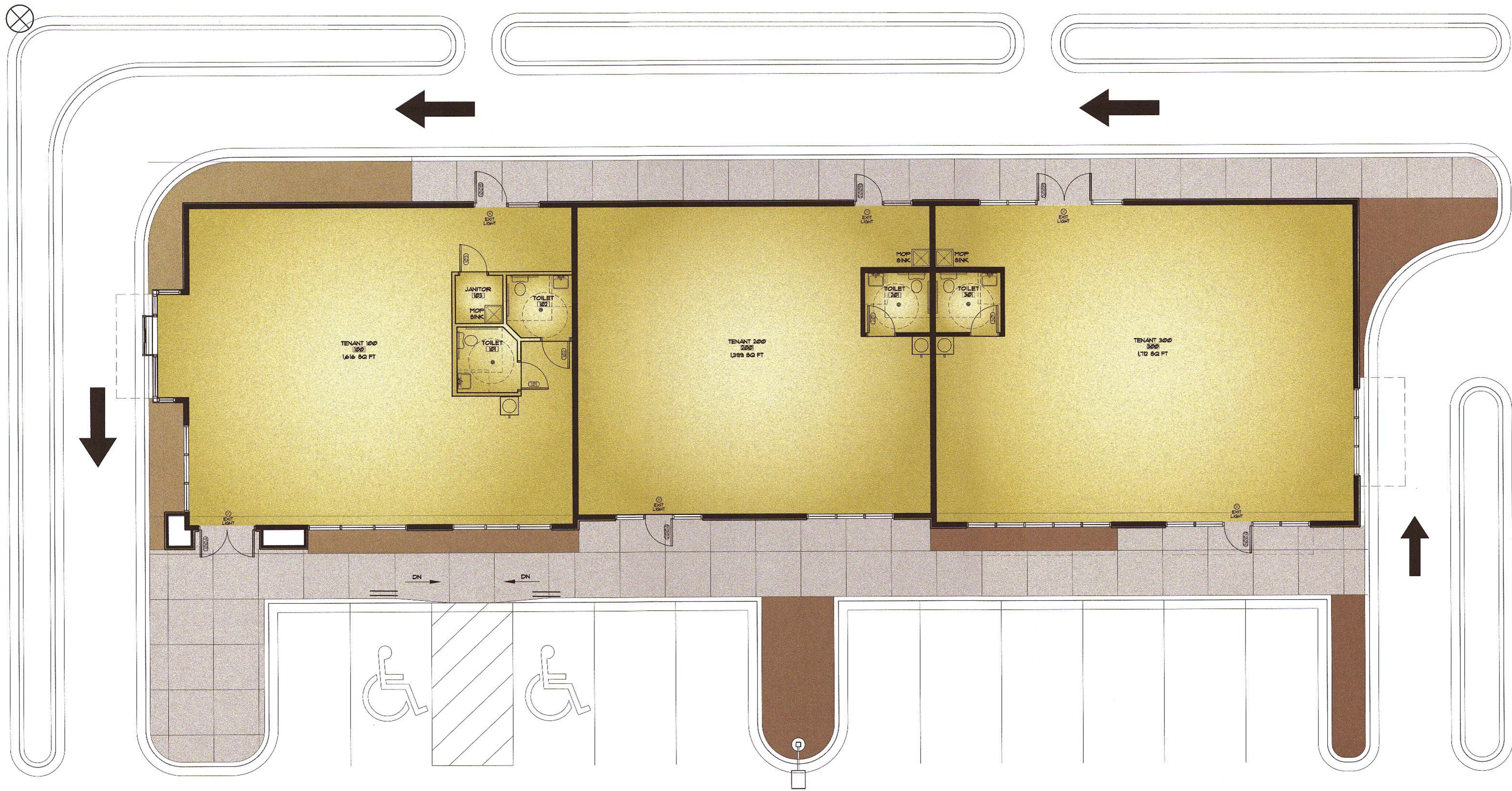
1 FLOOR PLAN SCALE: 3/16" = 1' - 0" 4,727 SQ. FT. NORTH
