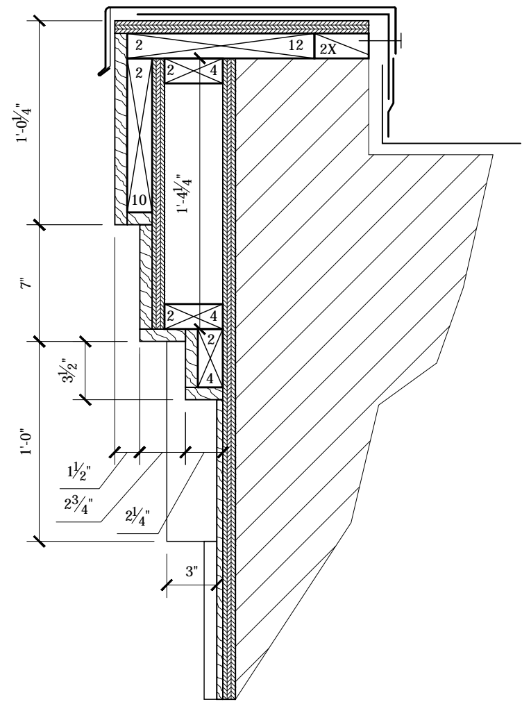
1 COPING PROFILE A NTS
