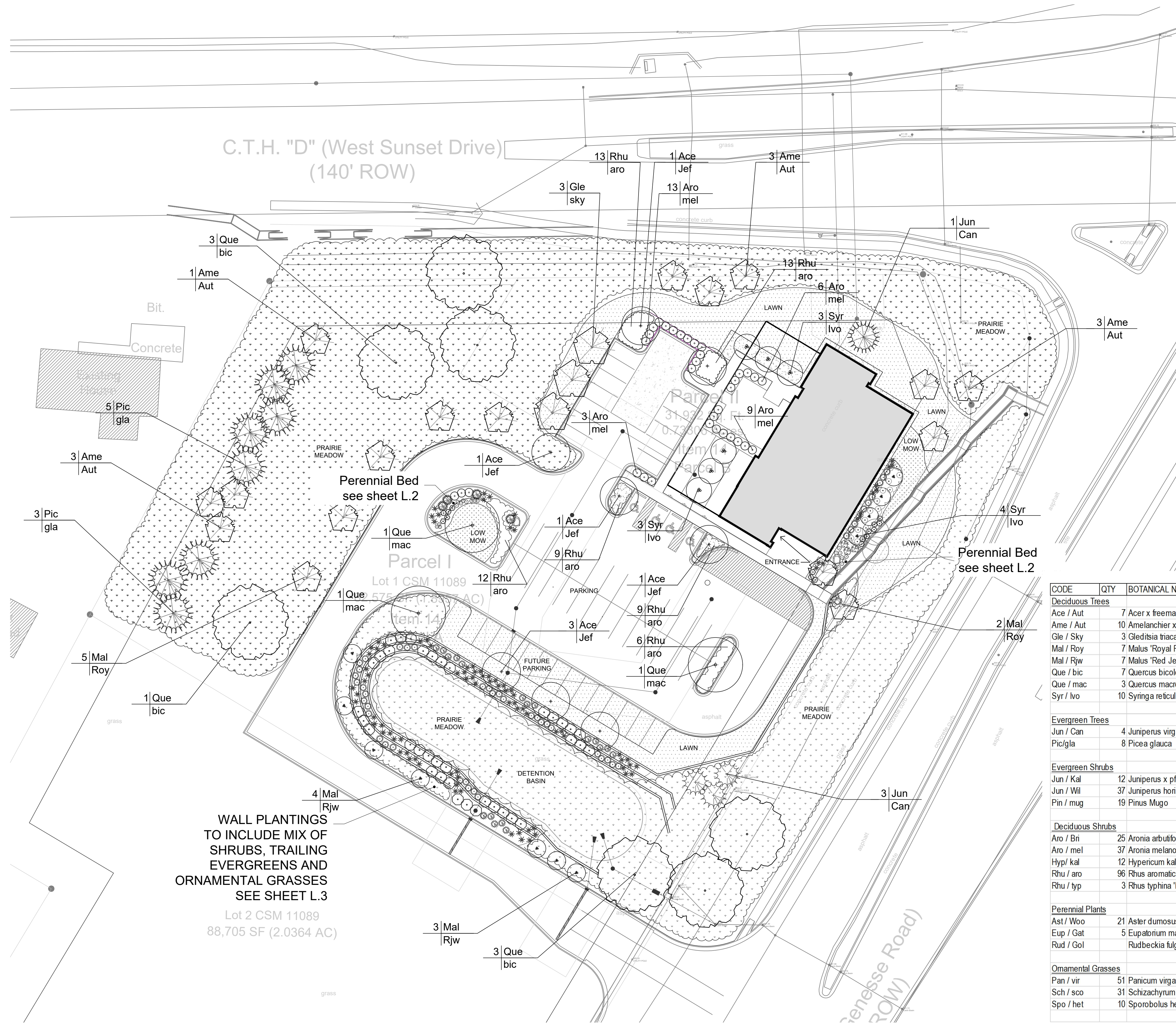
PLANT SCHEDULE
