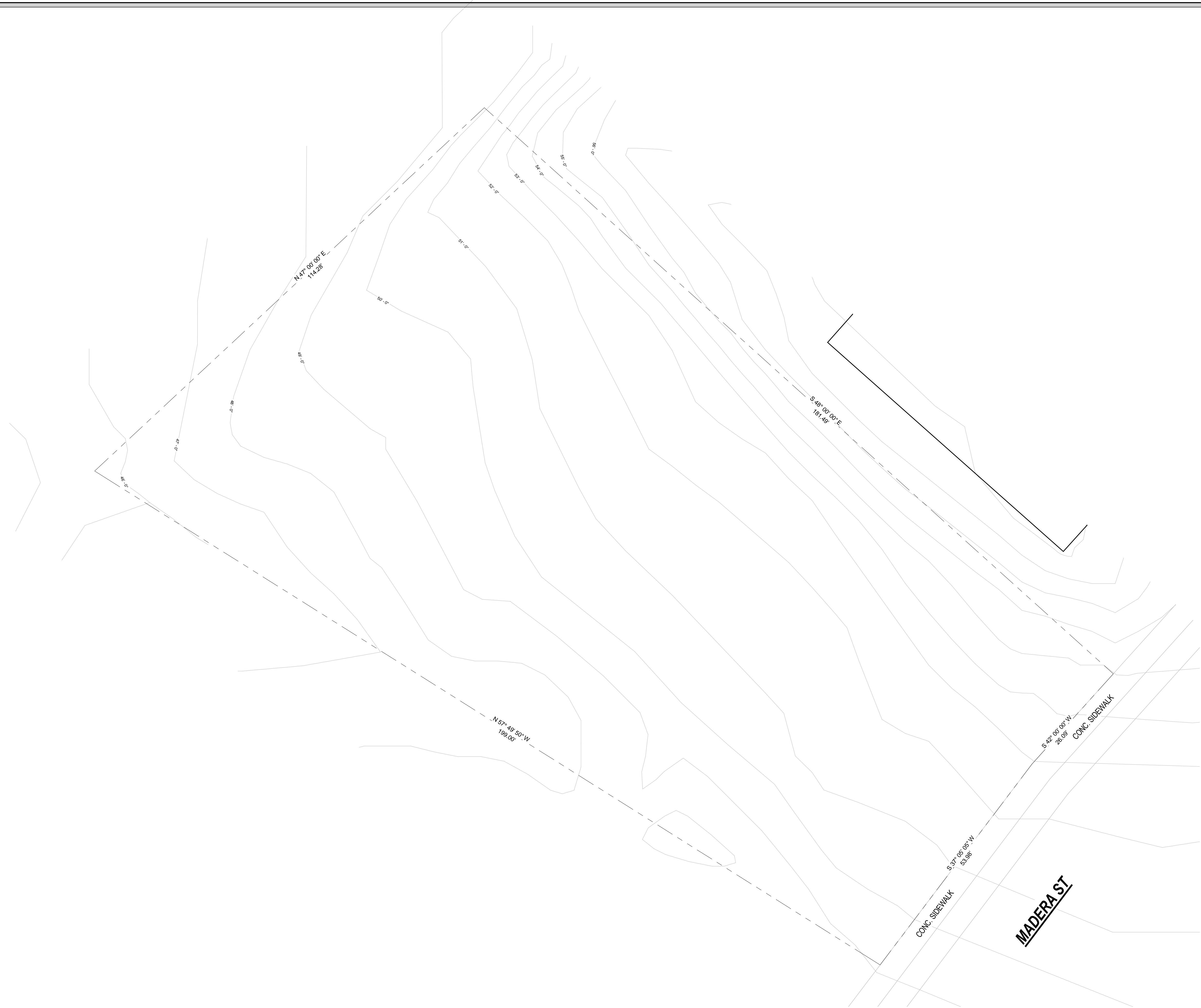
3 EXISTING GRADING PLAN 1" = 10'-0"
