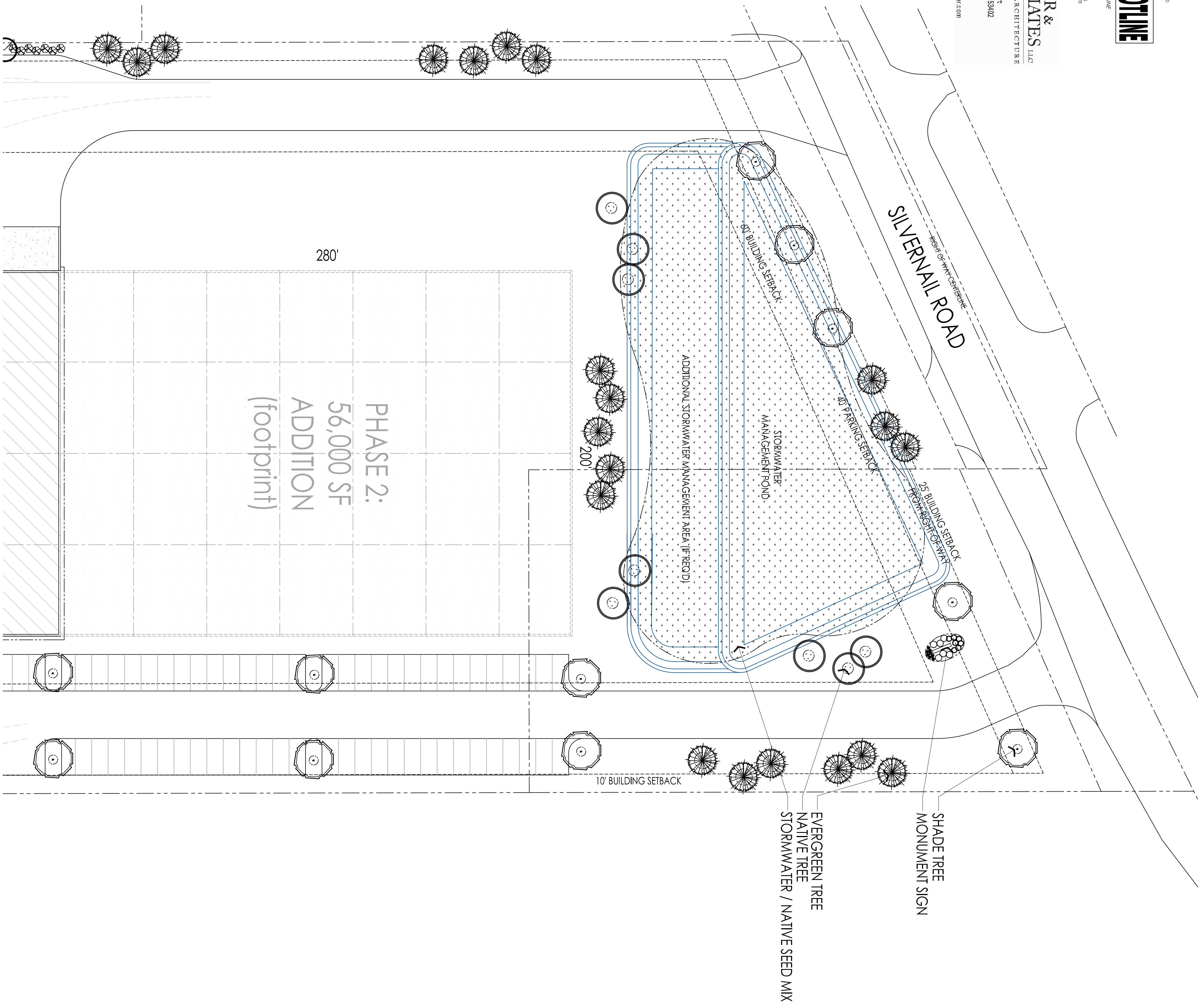
LANDSCAPE PLAN ENLARGEMENT - NORTH SCALE: 1"=300"
