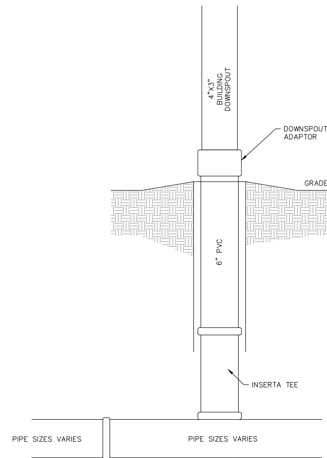
DOWNSPOUT DETAIL
