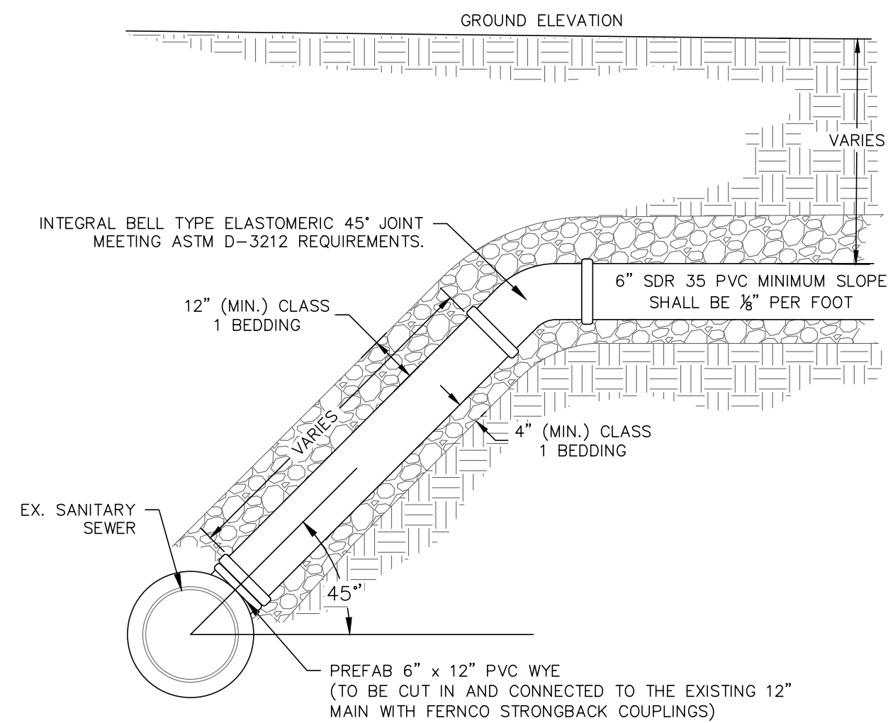
SANITARY LATERAL RISER DETAIL
