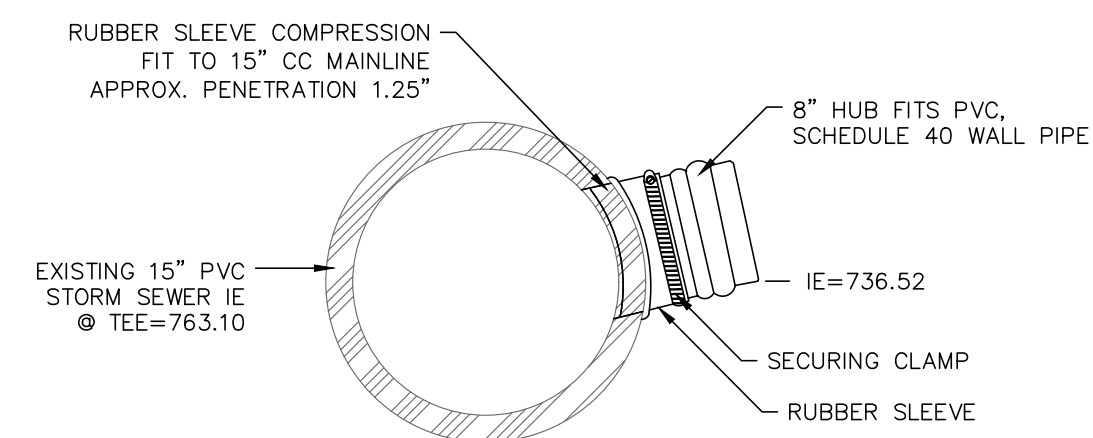
INSERTA TEE DETAIL
