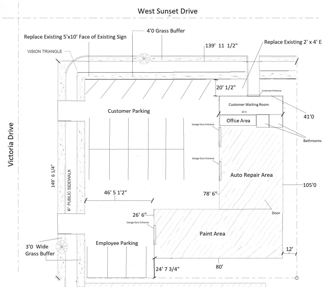
1 Landscaping Plan 1" = 20'-0"
