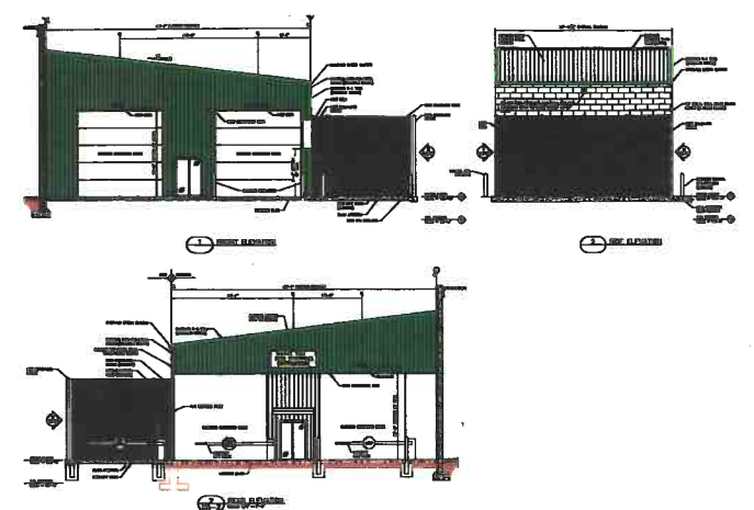
2 YARD ENTRANCE ADDITION SCALE: 1/16" = 1'-0"
