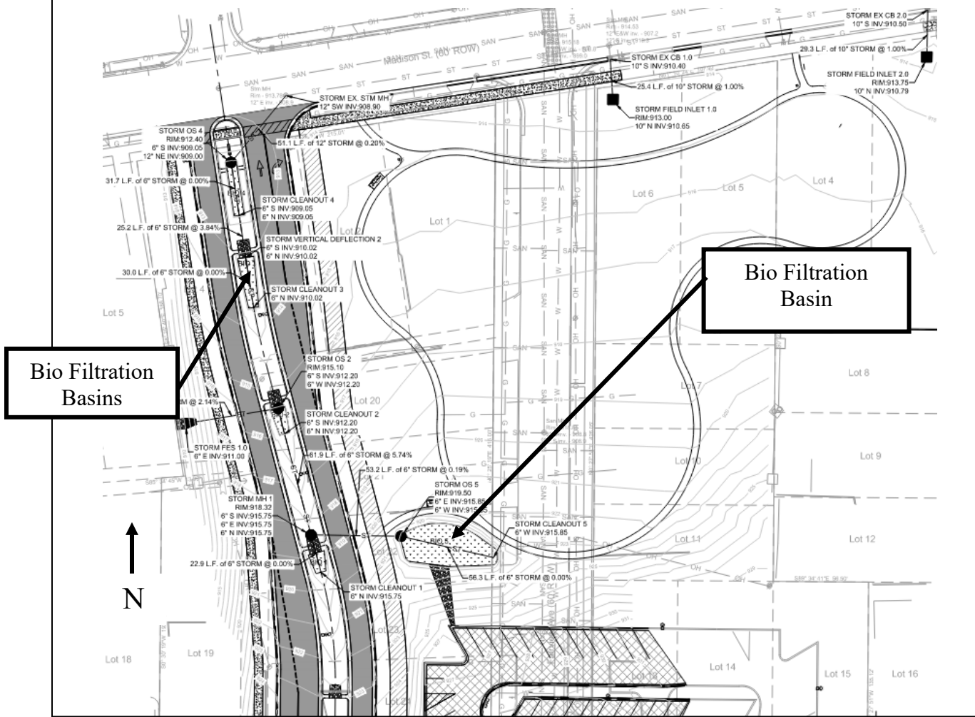
Plan View of Storm Water Practices
