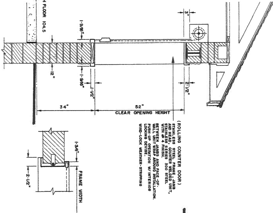
DETAIL THRU CONCESSION COUNTER THRU DOOR SCALE 3/4" = 1'-0"
