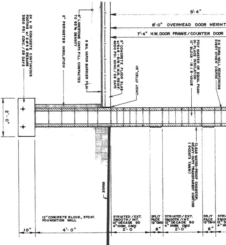
DETAIL SECTION THRU BUILDING WALLS SCALE 3/4" = 1'-0"
