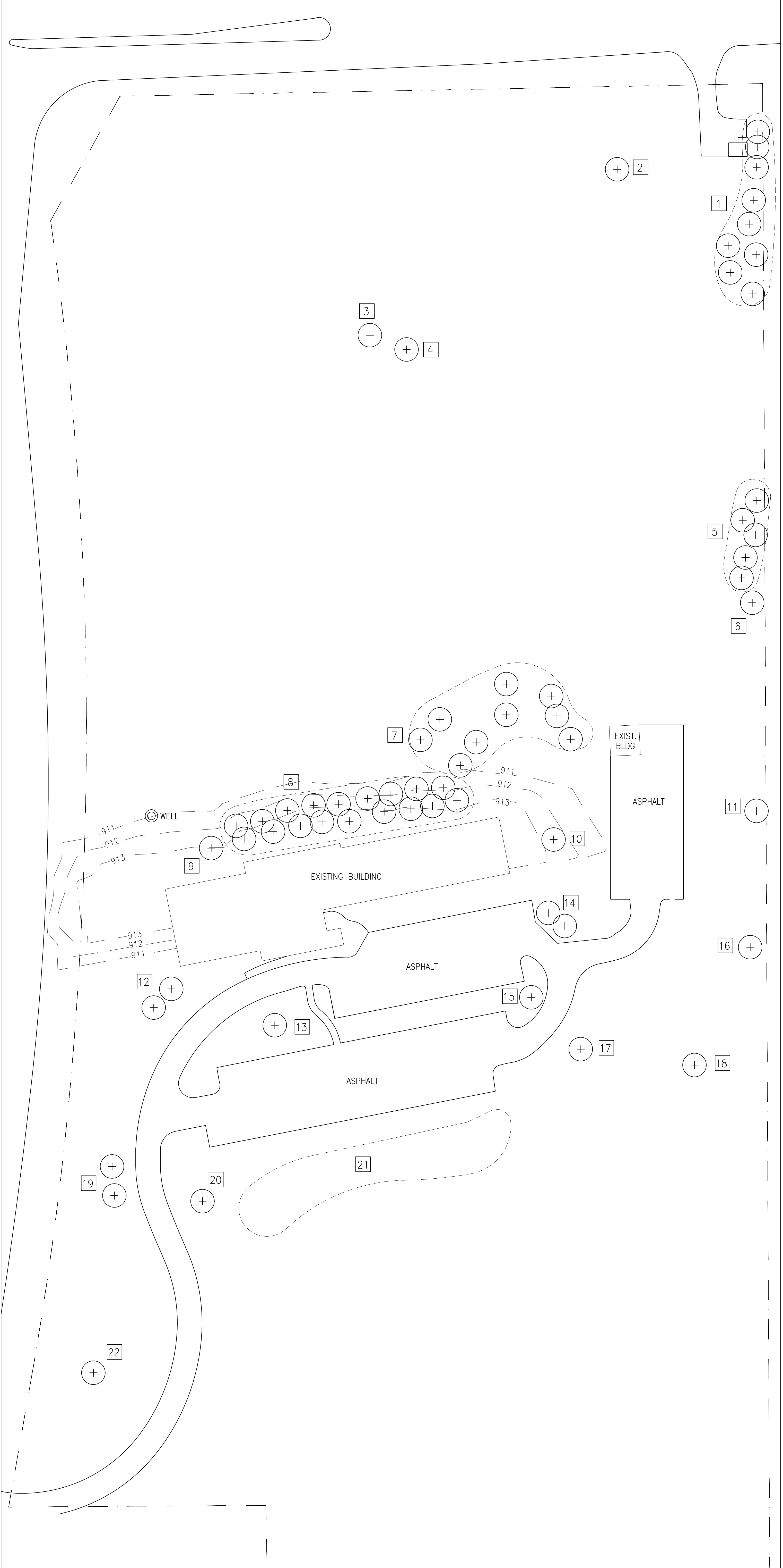
TREE INVENTORY 1"=40'-0"
