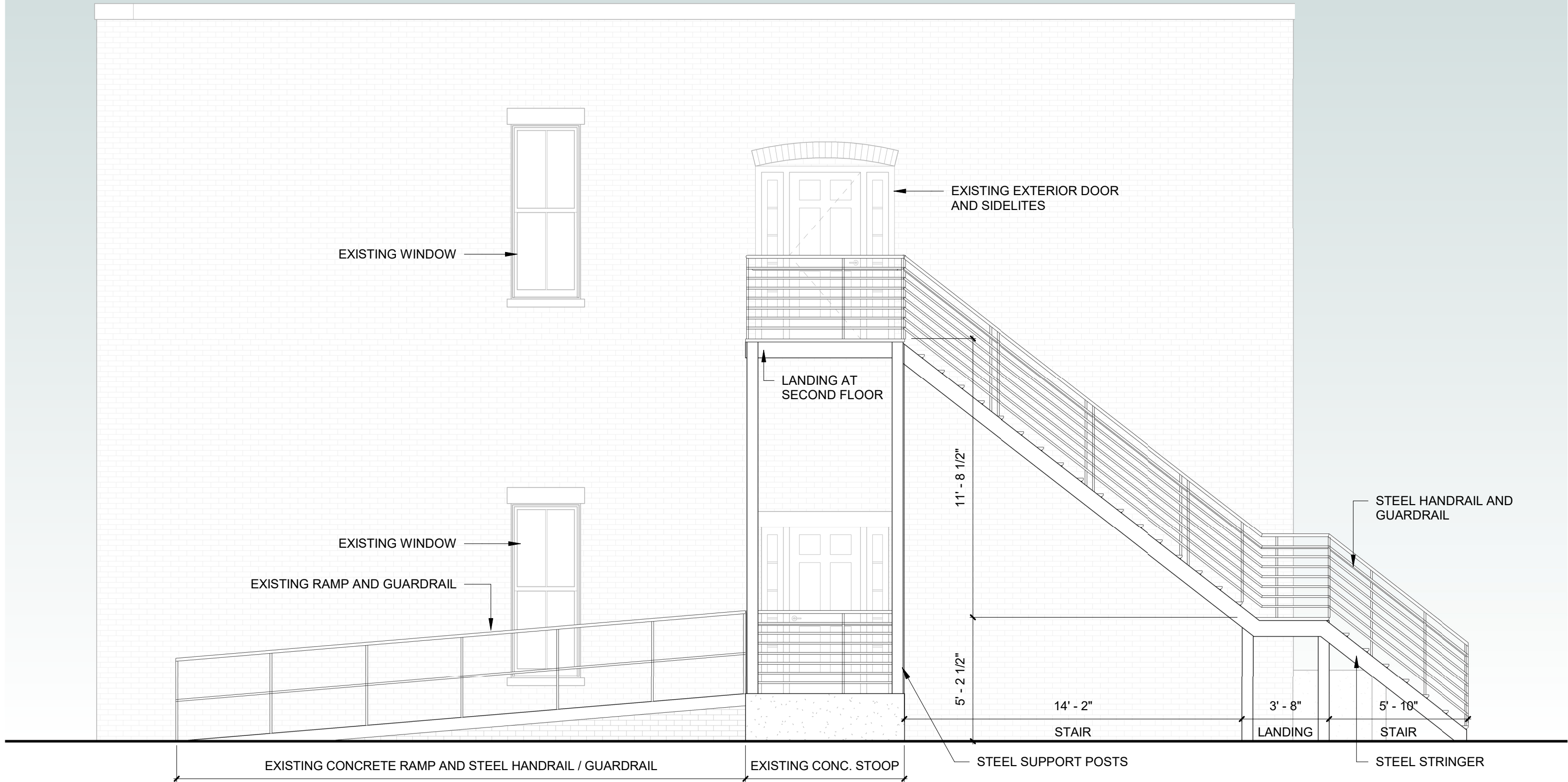
1 South Elevation 1/4" = 1'-0"
