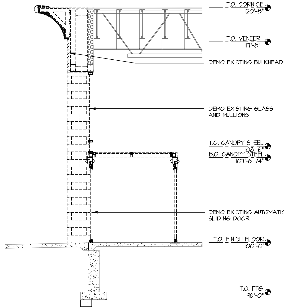
2 DEMO WALL SECTION 1/4" = 1'-0"
