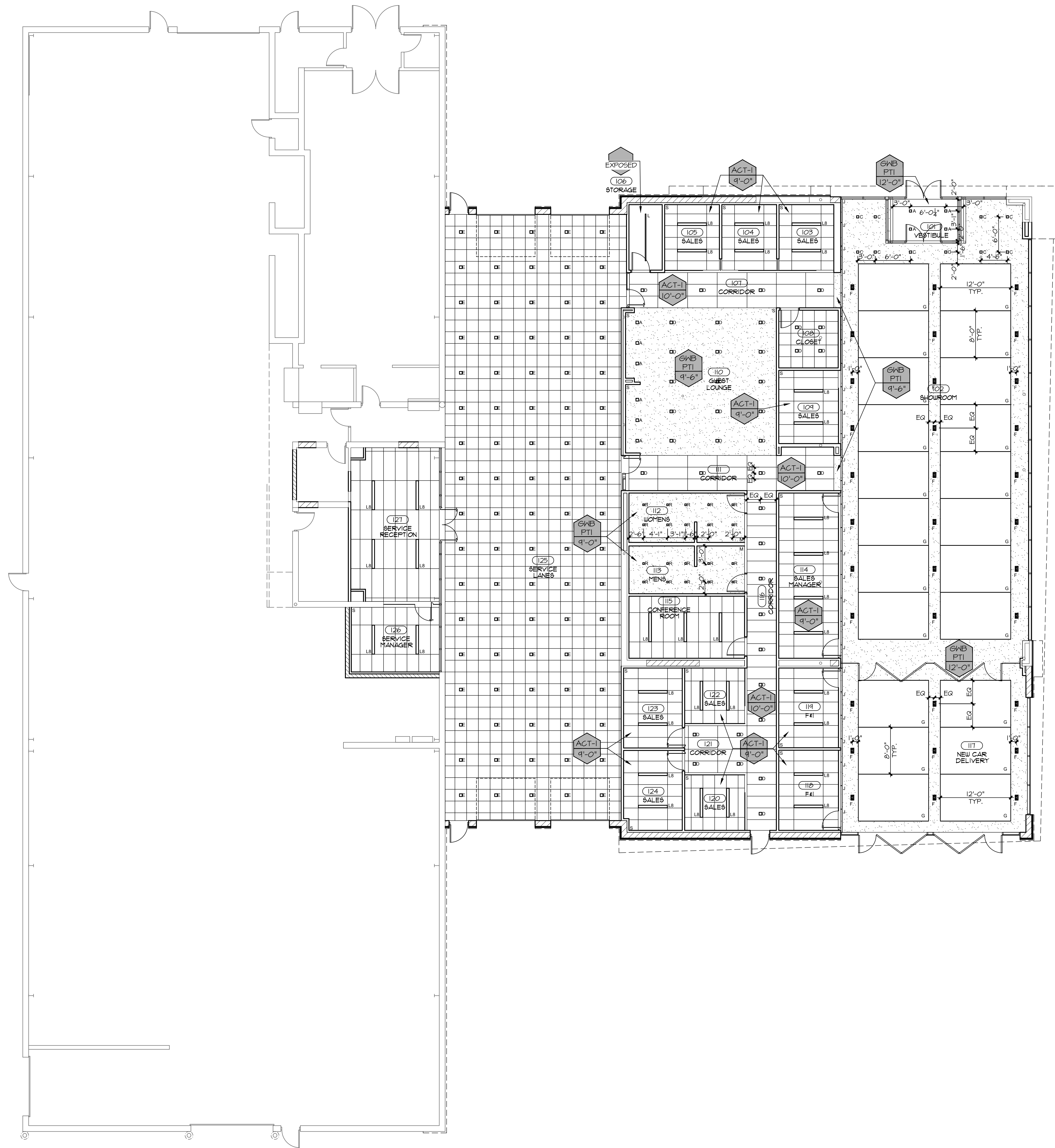
1 FIRST FLOOR REFLECTED CEILING PLAN 1/8"=1'-0" NORTH
