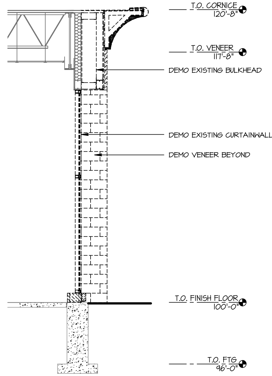
1 DEMO WALL SECTION 1/4" = 1'-0"
