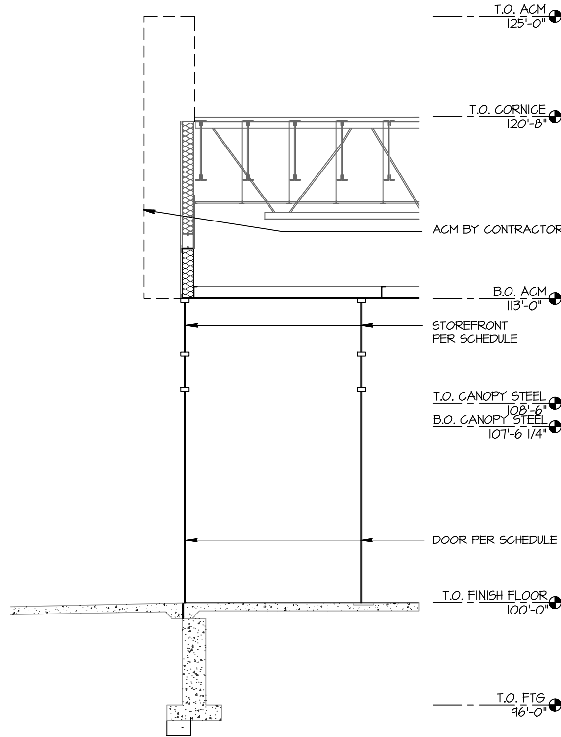
4 WALL SECTION 1/4" = 1'-0"
