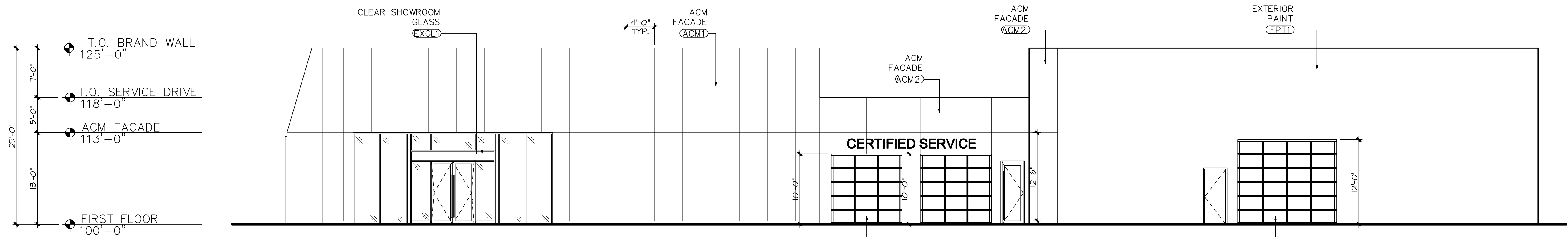
2 EAST ELEVATION 1/8" = 1'-0"
