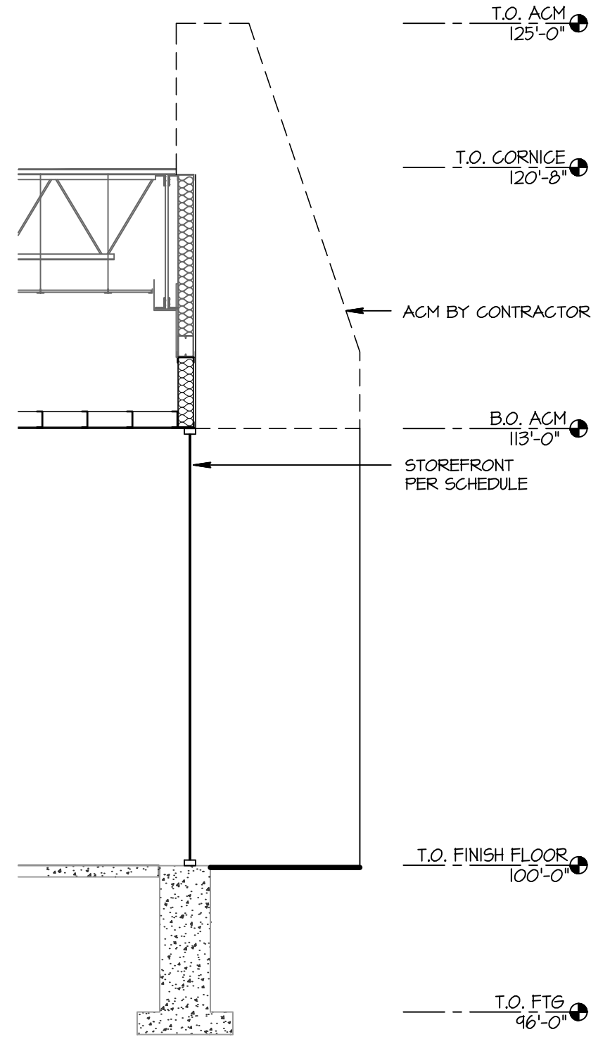
3 WALL SECTION 1/4" = 1'-0"
